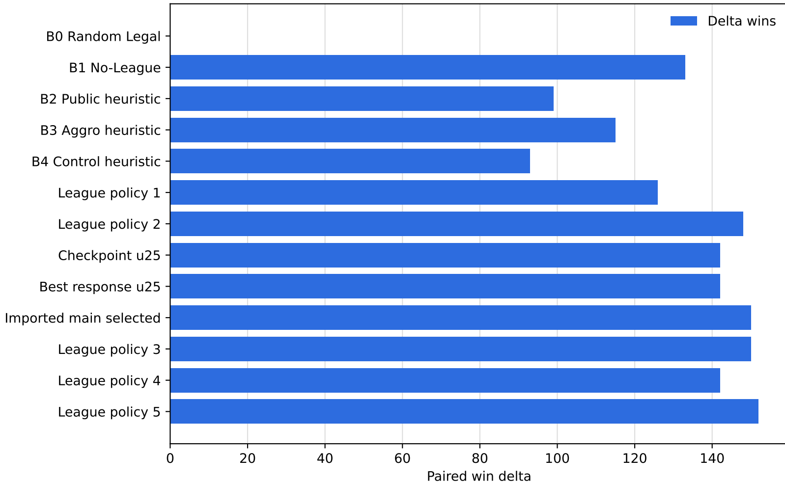
Search-enhanced main paired win deltas
