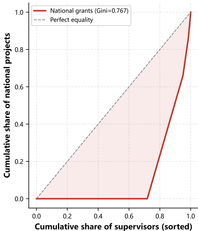
(a) Lorenz Curve: National Project Allocation (Gini = 0.767, Top 5% hold 34.0%)
