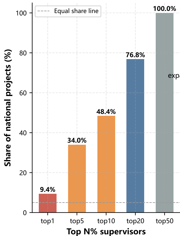
(b) Pareto Concentration (Top 20% supervisors hold 76.8%)
