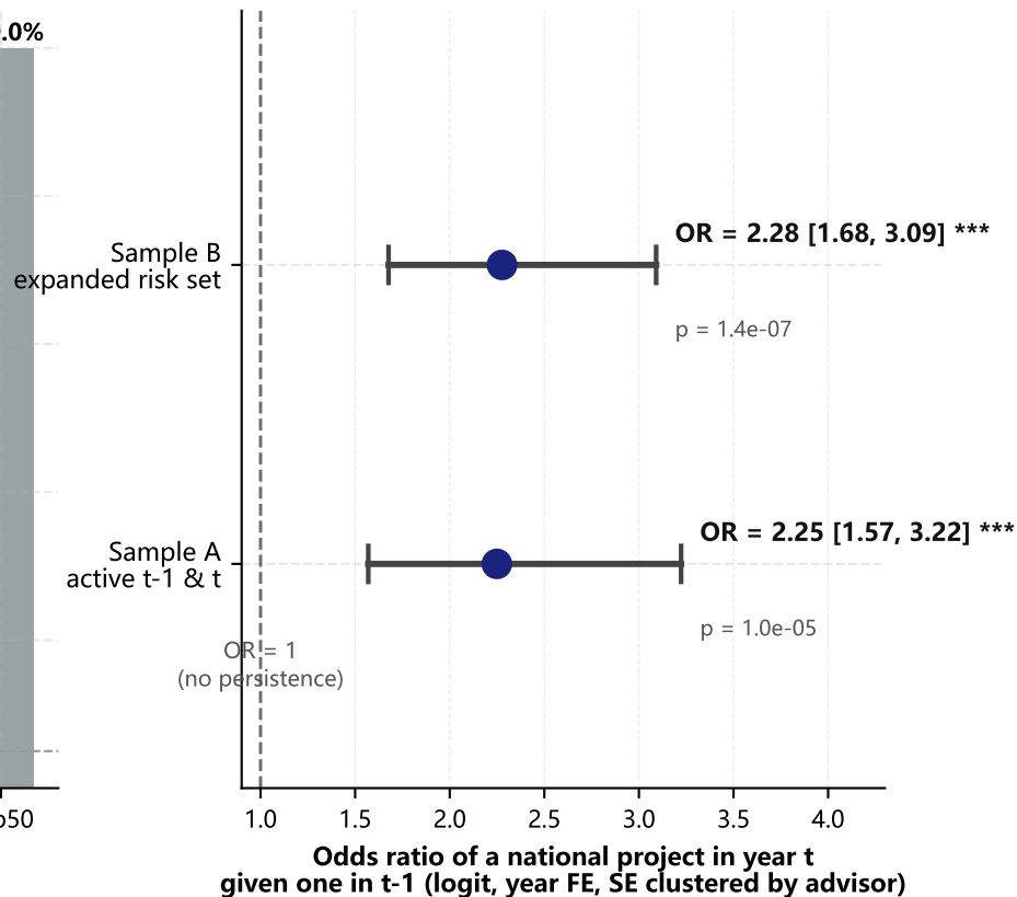
(c) Path Dependence: Lagged Logistic (national project persistence t-1 -> t)
