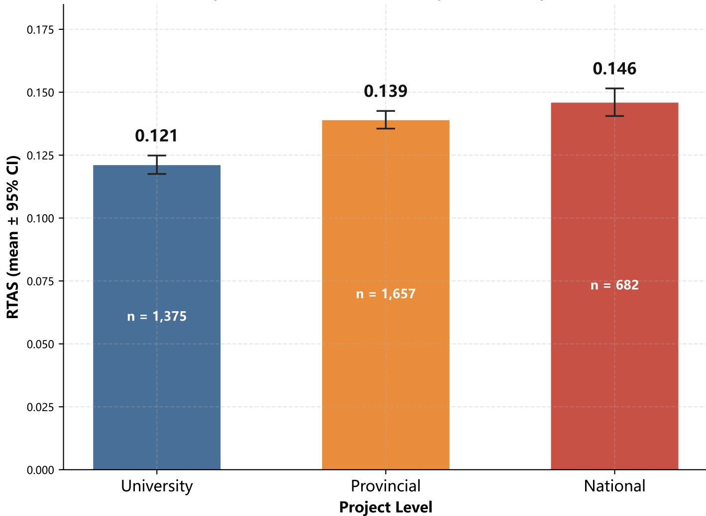
(a) Mean Research-Training Alignment Score by Project Level One-way ANOVA: F(2, 3711) = 35.72 , p = 4.3e-16 , \eta^2 = 1.89\%
