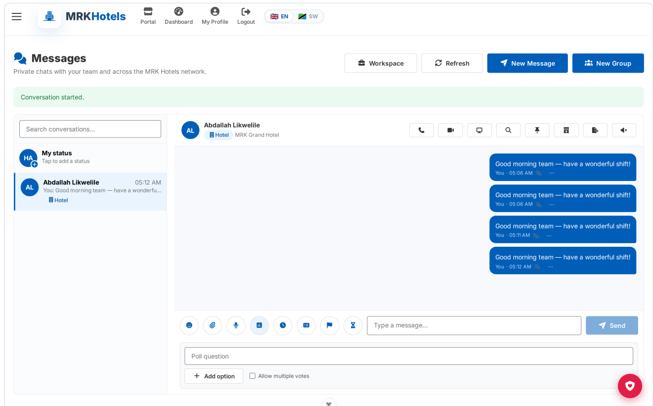
Composer tools — poll builder, scheduler and template picker.
