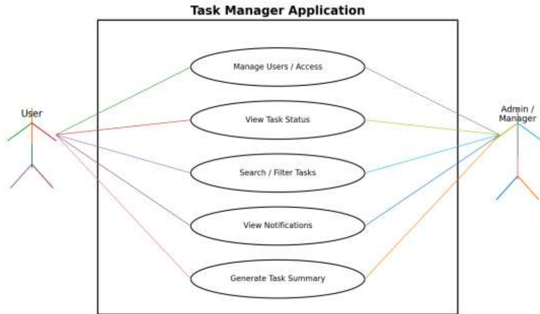
Figure 2. UML Use-Case Diagram: Monitoring and Administration
