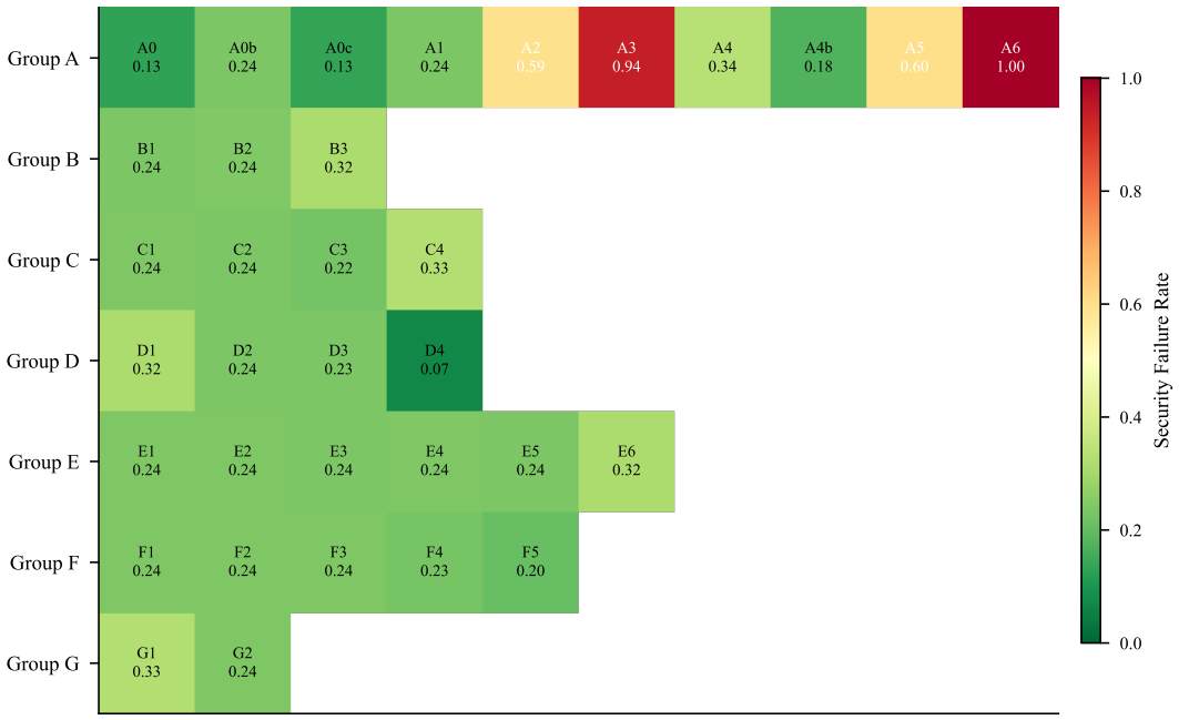
Security Failure Rate by Experiment
