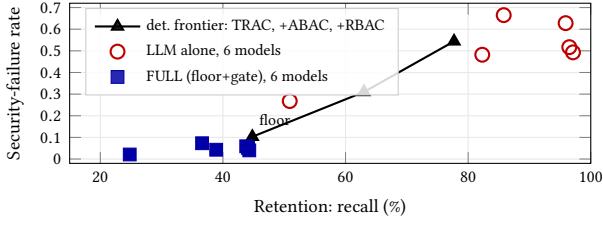
Figure 2: Operating-point map: security-failure rate vs. retention (recall, % of domain-eligible requests admitted). The model-independent deterministic frontier (TRAC \rightarrow +ABAC \rightarrow +RBAC) is monotone; every LLM-only validator sits well above it at high security-failure regardless of retention, while composing each model’s verdict behind the floor (FULL) pulls all six models, across three vendors, into a tight low-security-failure cluster ( \leq 7.3\% ), none exceeding the 10.3% floor. Retention counts every denied domain-eligible request, including intended least-privilege denials by RBAC/ABAC; policy-conditioned availability (admissible-only) is higher (80.7%, §6.1). Values: Table 10; replay via scripts/sweep_op_points.py .
