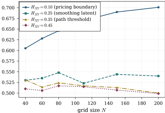
classification accuracy
