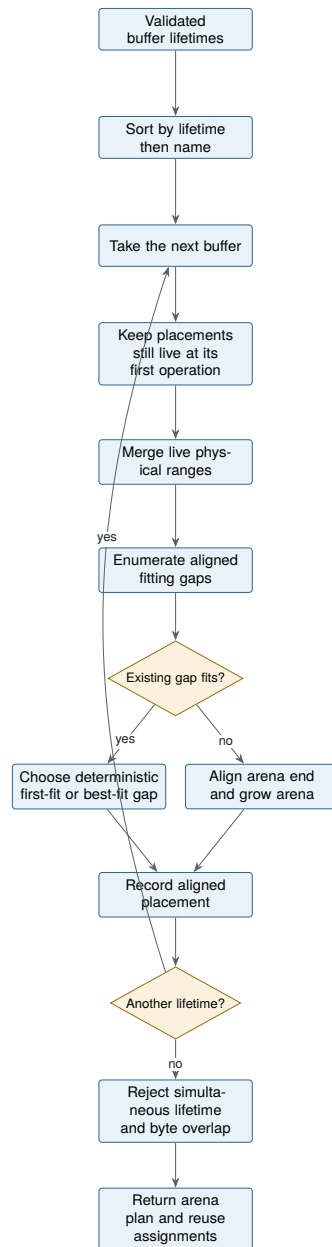
Figure 42.1: Lifetime arena planning.
