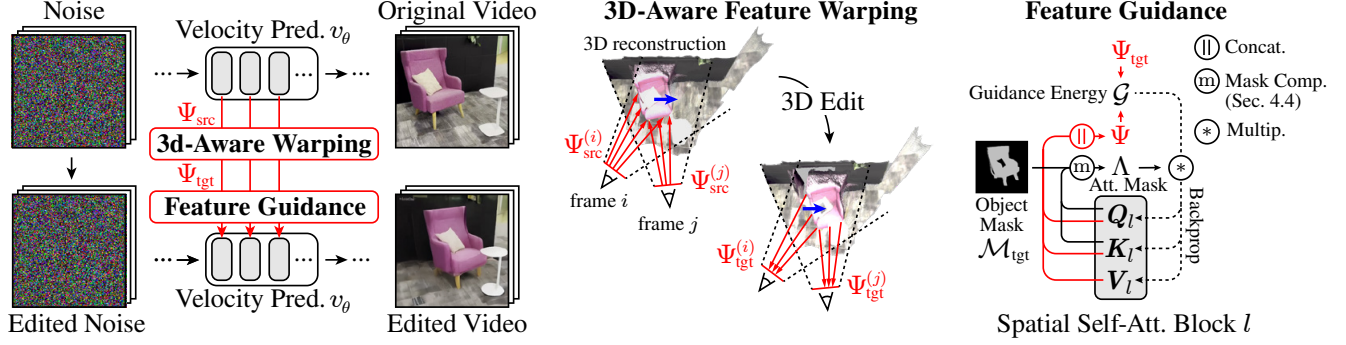
Figure 2. VideoHandles Architecture. We use the intermediate features \Psi_{src} of a video generative model to represent the identity of objects in a source video. Given a 3D transformation of an object, we can use a 3D reconstruction of the scene to warp the intermediate features consistently across frames. Guiding the video generator with these warped features \Psi_{tgt} gives us an edited video where the object is transformed, while also maintaining the plausibility of effects like shadows and reflections.
