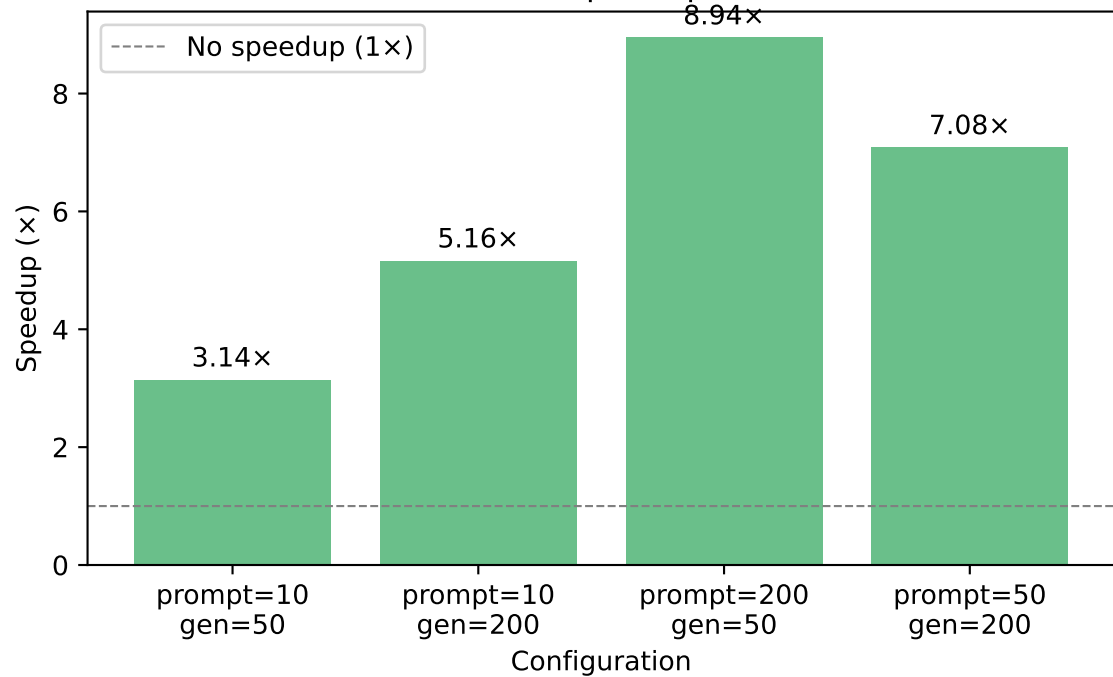
KV-Cache Speedup Ratio
