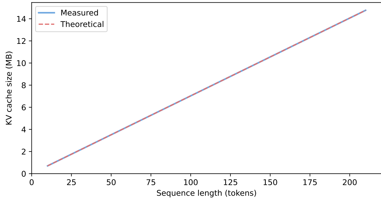
KV Cache Memory Growth
