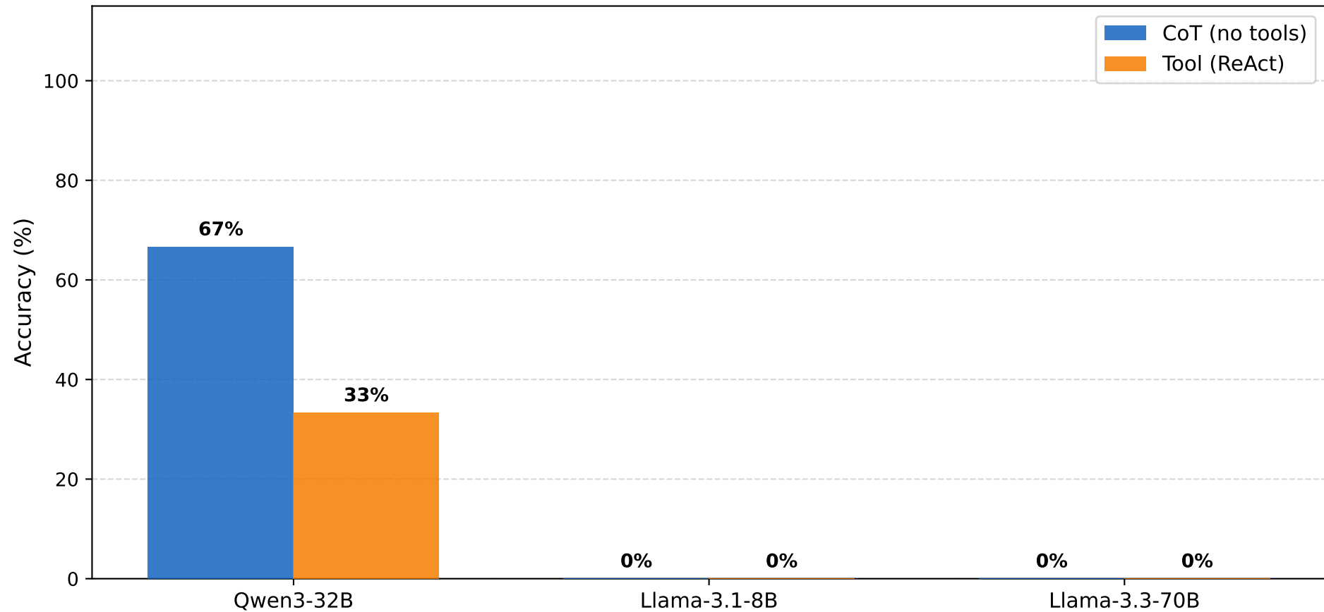
Accuracy per Model: CoT vs Tool Calling
