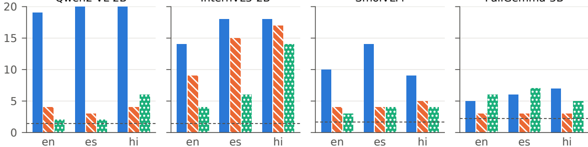
Qwen2-VL-2B
