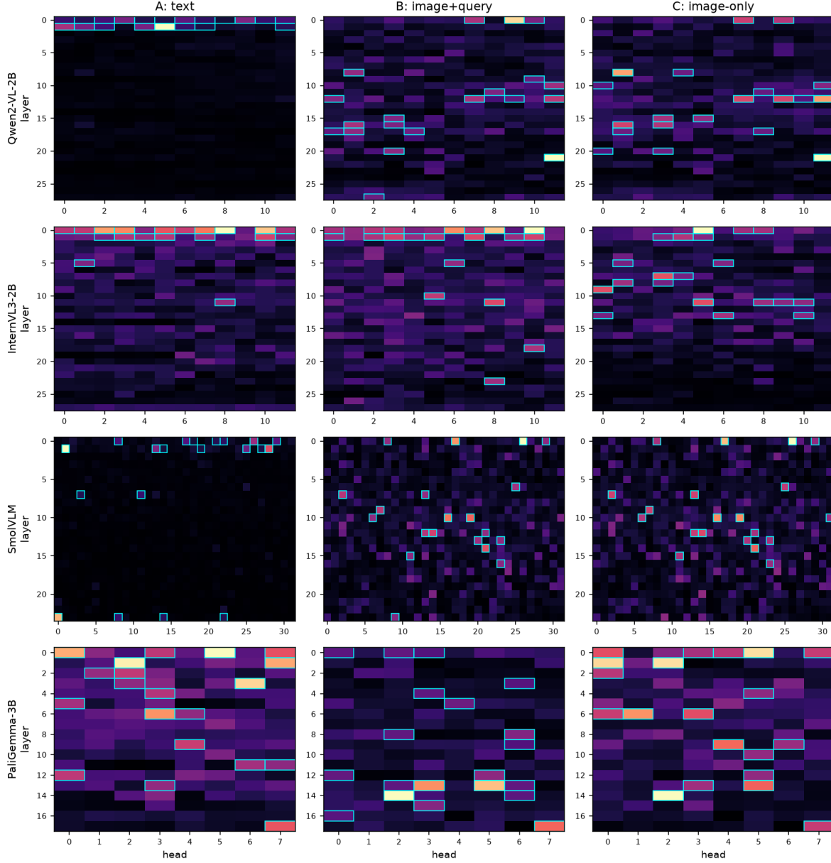
Figure 9: LAHIS head importance for Spanish, plotted as in Figure 8. The important heads lie in the same layers as for Hindi, but InternVL3-2B’s text and image panels agree less than for Hindi.
