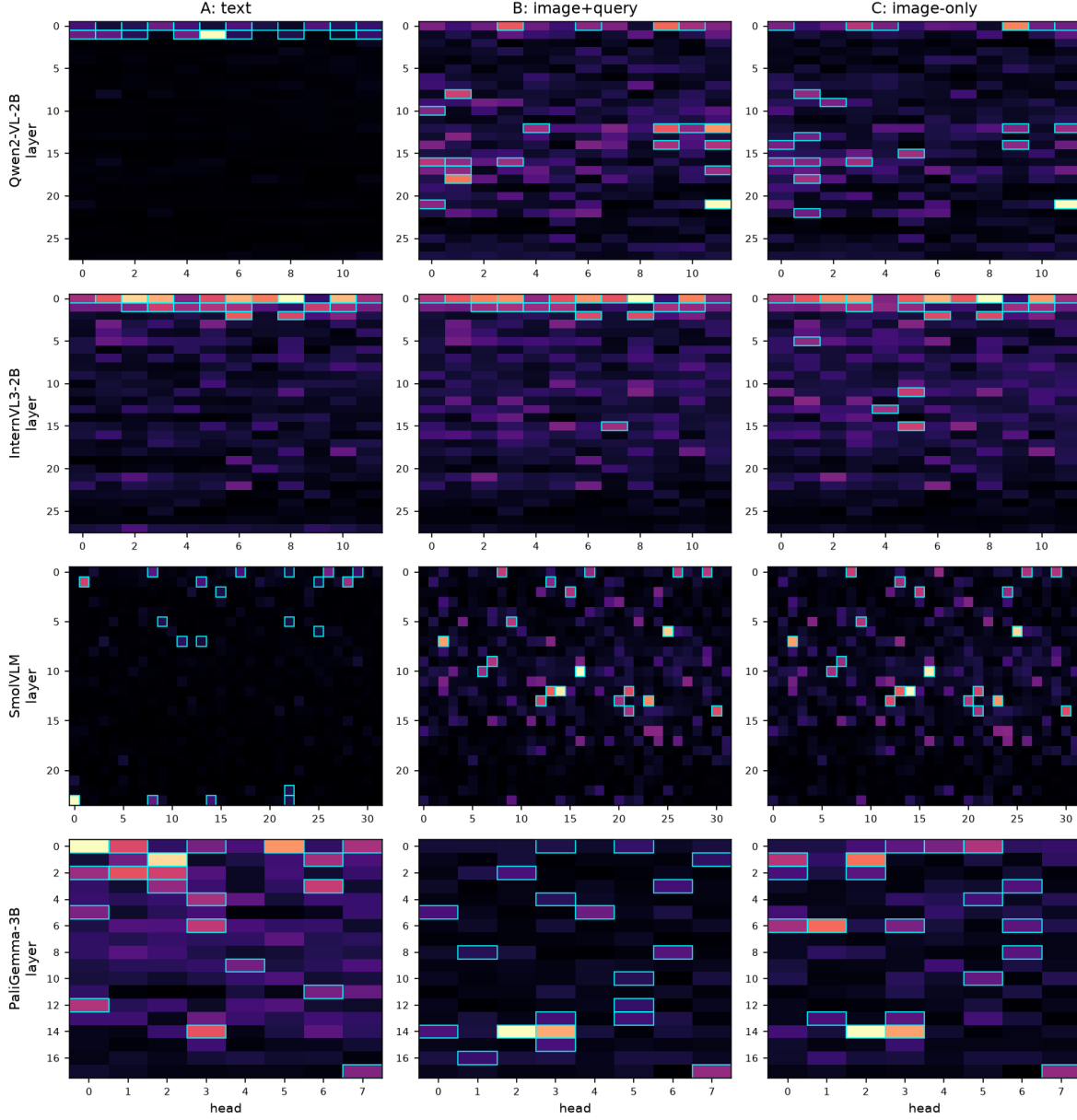
Figure 8: LAHIS head importance for Hindi. Rows are models and columns are input conditions. Cyan rings mark each panel’s top 20 heads, and scores are min-max normalized within each panel. Qwen2-VL-2B’s text-condition heads lie in the first two layers while its image-condition heads spread through the network, and InternVL3-2B’s three conditions highlight the same early heads.
