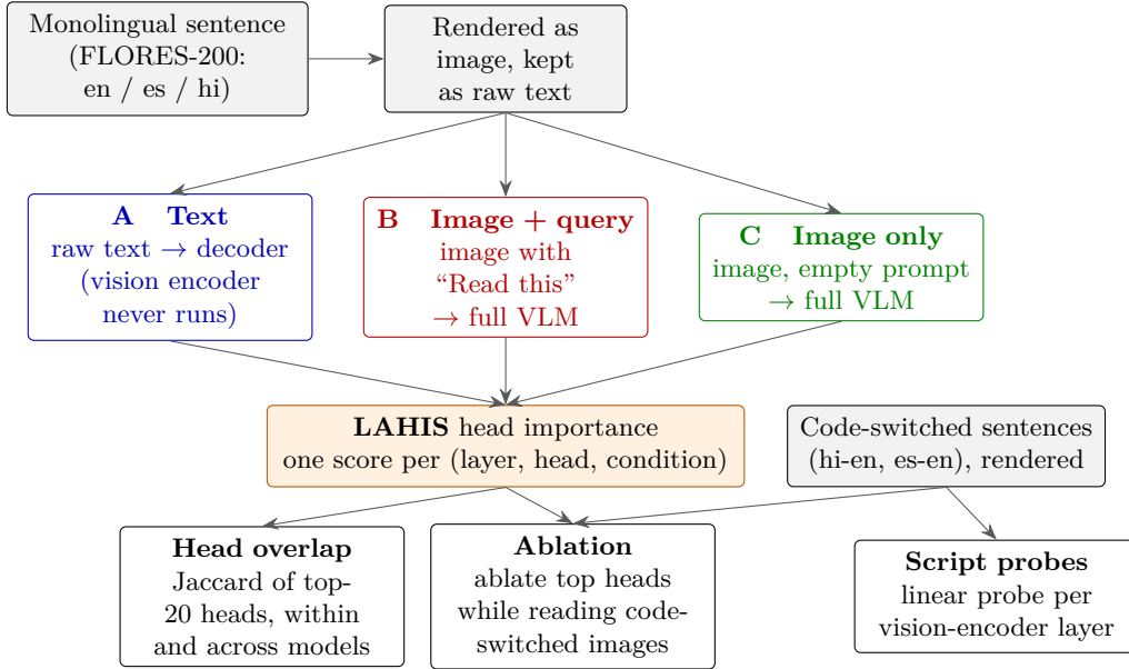
Figure 3: Overview of the pipeline. (Top) Each monolingual sentence is scored with LAHIS in three input conditions. (Bottom) The top heads are compared across conditions and models, and ablated while the model reads rendered code-switched sentences. The script probes use the same code-switched images.
