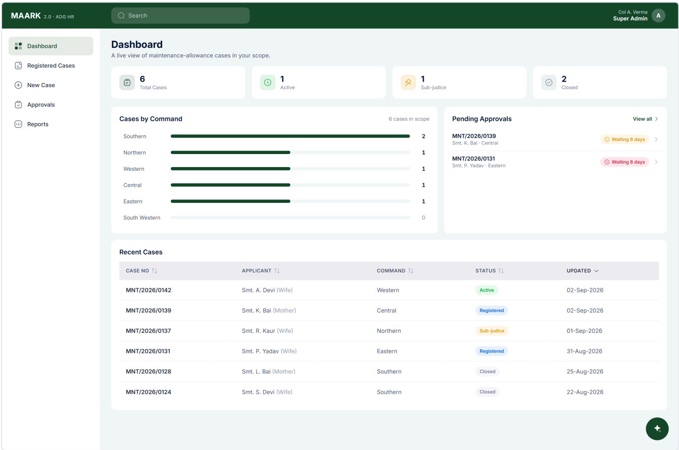
Figure 2 – Dashboard
