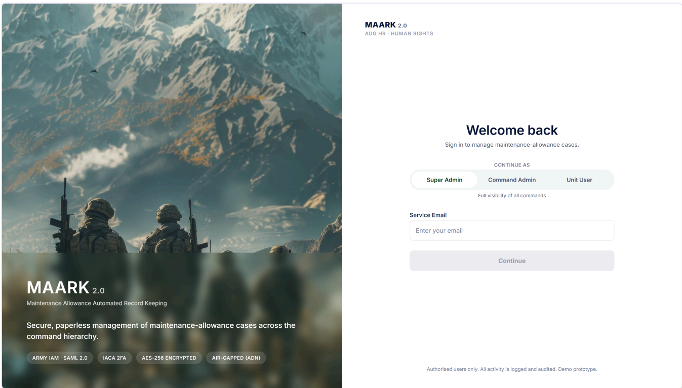
Figure 1 — Login
