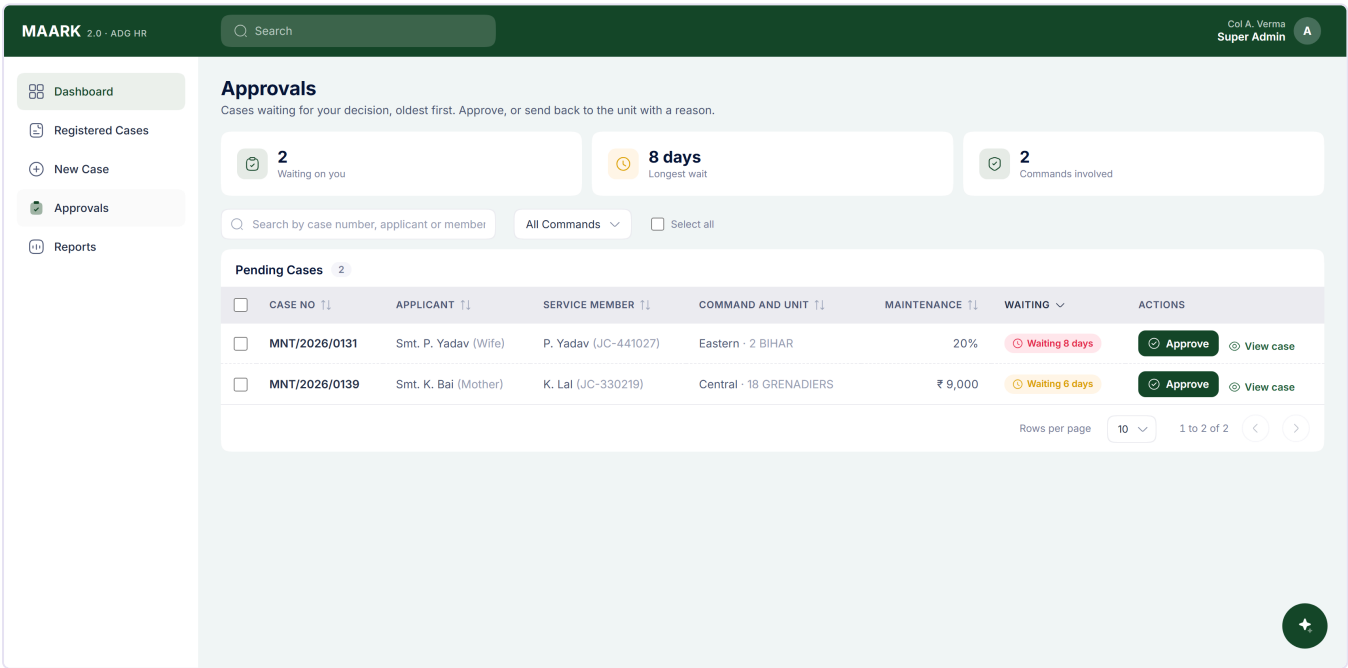
Figure 6 — Approvals queue
