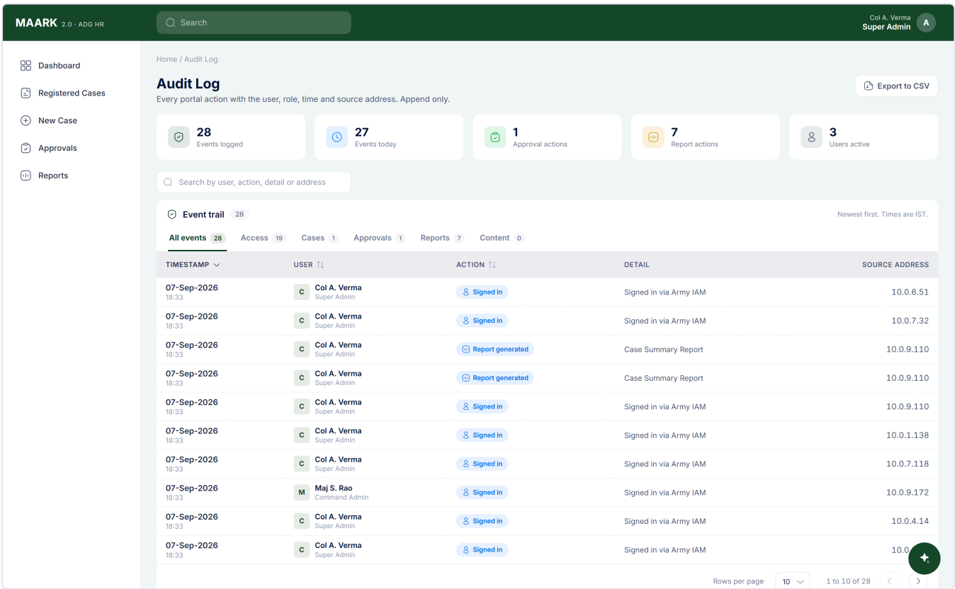
Figure 9 — Audit Log
