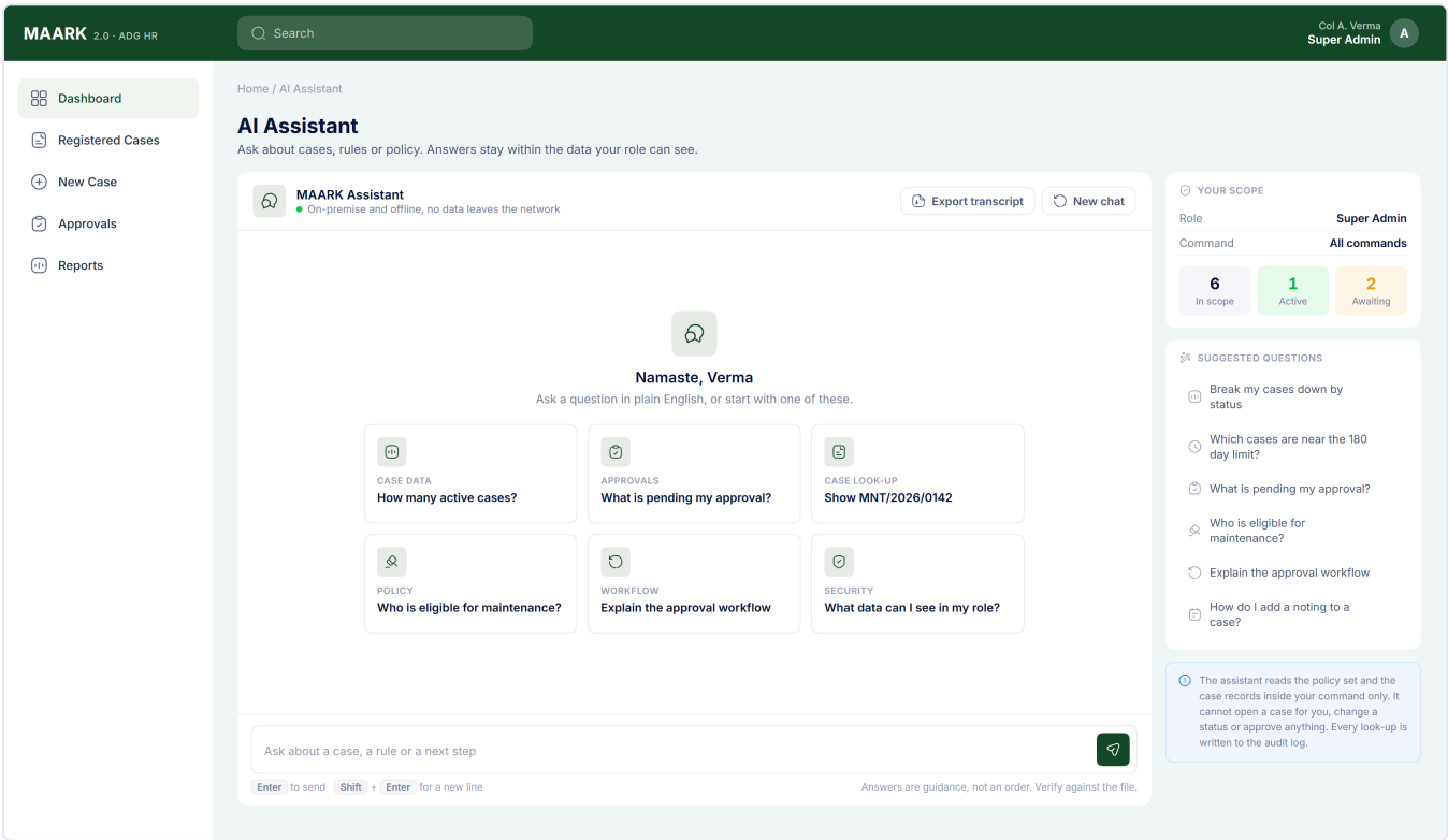
Figure 10 — AI Assistant
