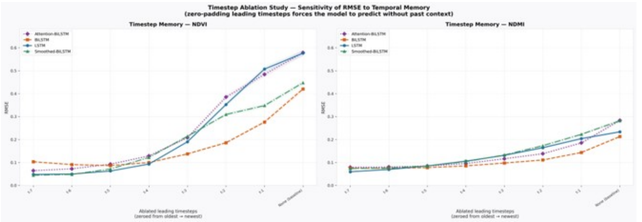
Figure 20: Timestep ablation study: RMSE sensitivity to temporal memory for NDVI (left) and NDMI (right).
