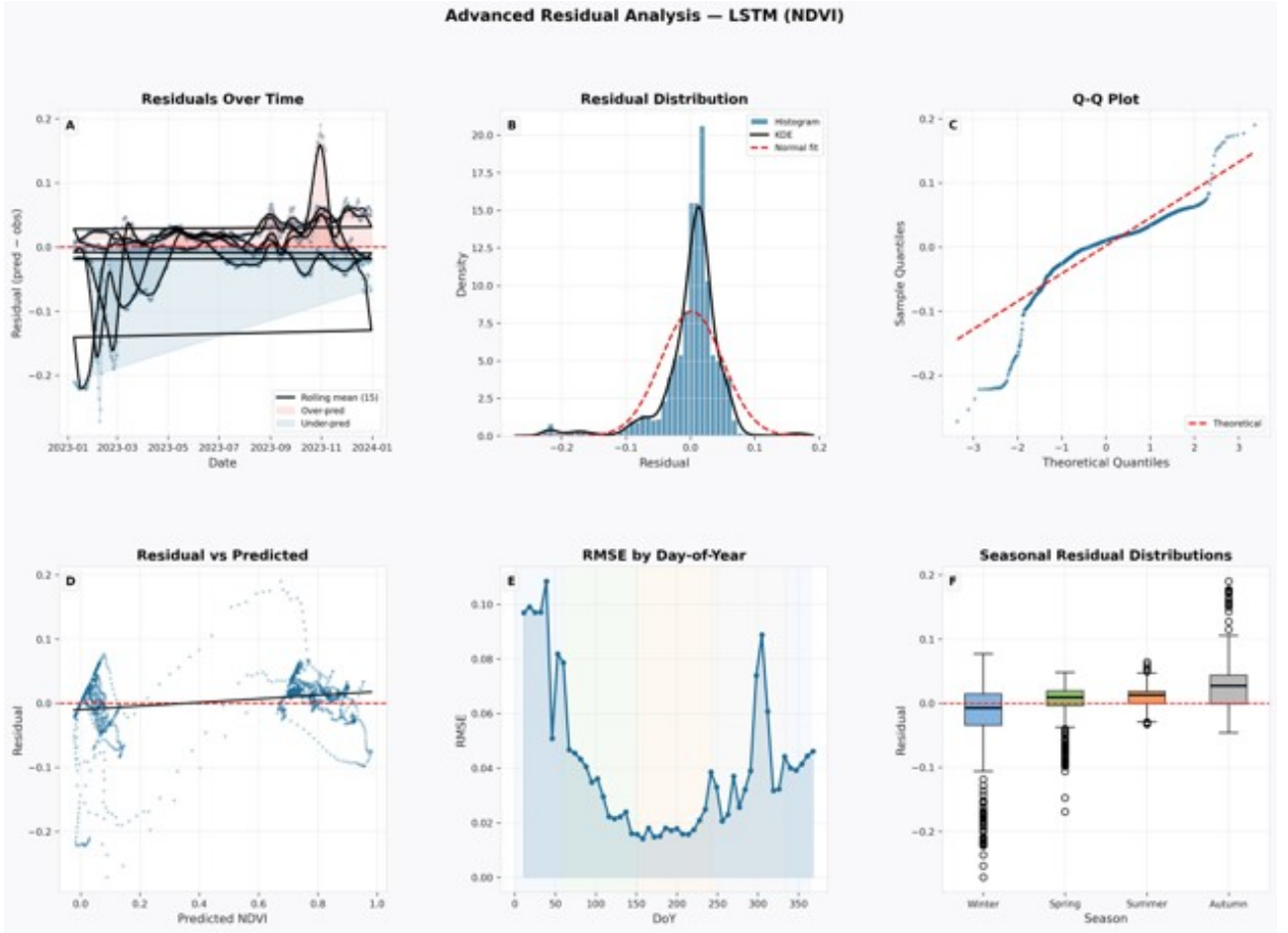
Figure 10: Advanced residual analysis for the LSTM (NDVI). Panels show: (A) residuals over time with rolling mean and over/under-prediction shading; (B) residual distribution with KDE and theoretical normal fit; (C) Q-Q plot; (D) residual vs. predicted value; (E) RMSE by Day-of-Year; (F) seasonal residual distributions.
