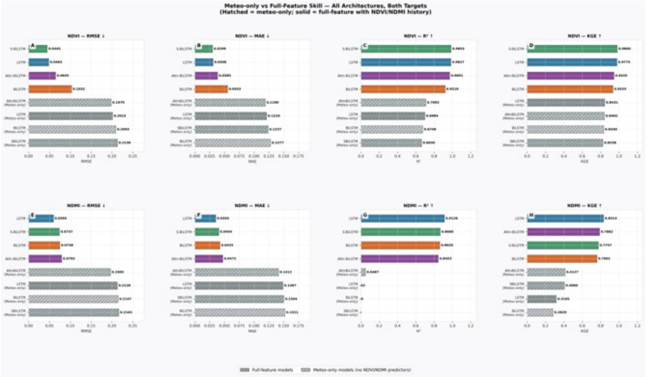
Figure 29: Meteo-only versus full-feature skill comparison for all architectures and both targets. Solid bars represent full-feature models; hatched bars represent meteo-only models (no NDVI/NDMI history).
