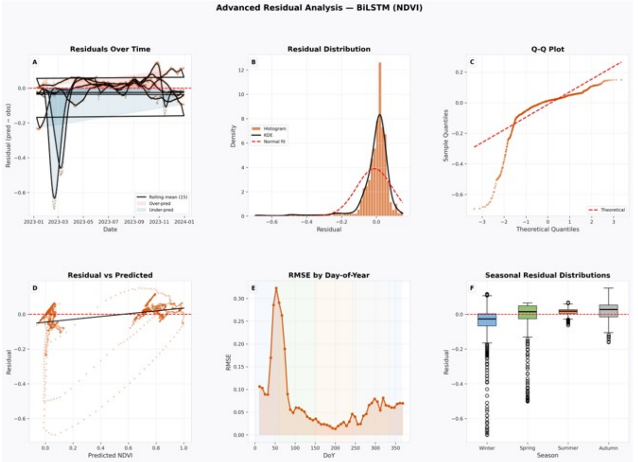
Figure 11: Advanced residual analysis for the BiLSTM (NDVI). Note the substantially wider residual range (panels A, B) and heavier tails in the Q-Q plot (C), indicating poorer distributional fit compared to the LSTM.
