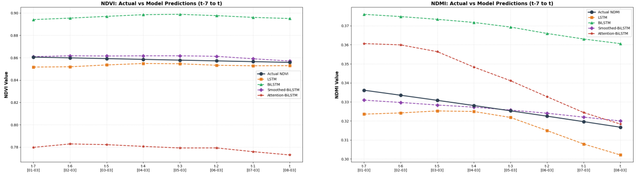
Figure 3: Sample execution of the 7-step sliding-window forecasting process for the period from 01 March 2023 to 08 March 2023 using the 21-predictor full feature set model.
