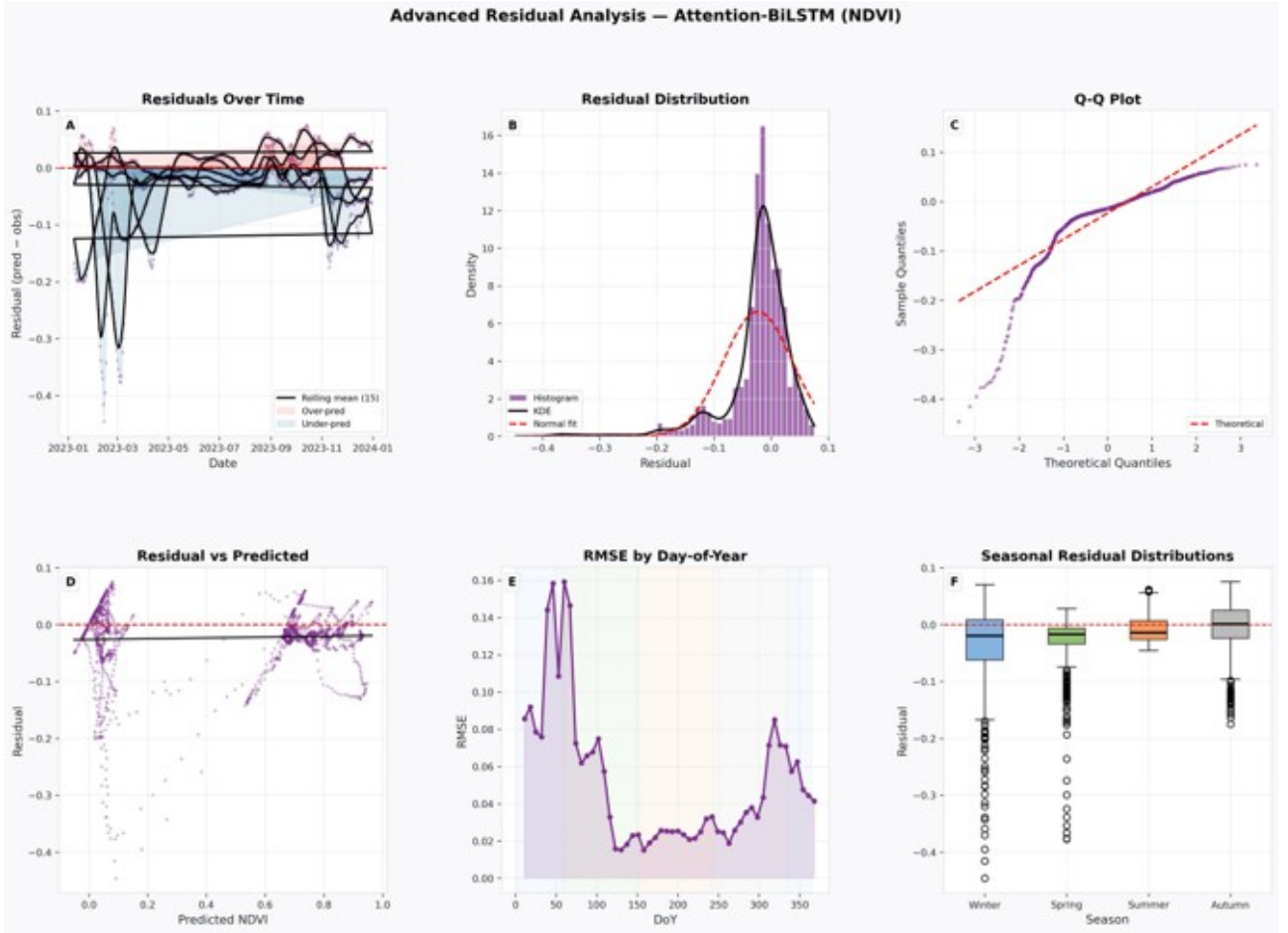
Figure 13: Advanced residual analysis for the Attention-BiLSTM (NDVI). The model displays persistent under-prediction bias (negative residuals), particularly during winter and spring, with a pronounced left-skewed residual distribution.
