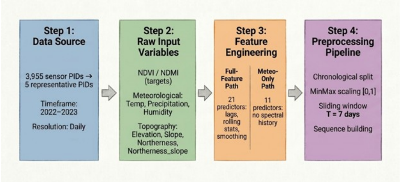
Figure 1: Input Data Preparation, Preprocessing & Processing
