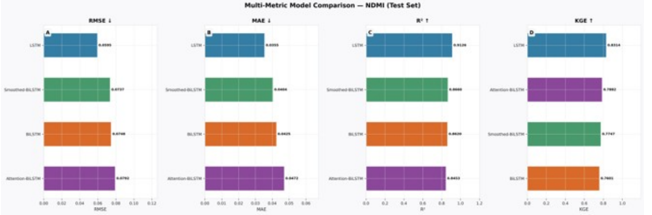
Figure 7: Multi-metric model comparison for NDMI prediction on the test set ( n = 1,790 ), showing RMSE (A), MAE (B), R^2 (C), and KGE (D).
