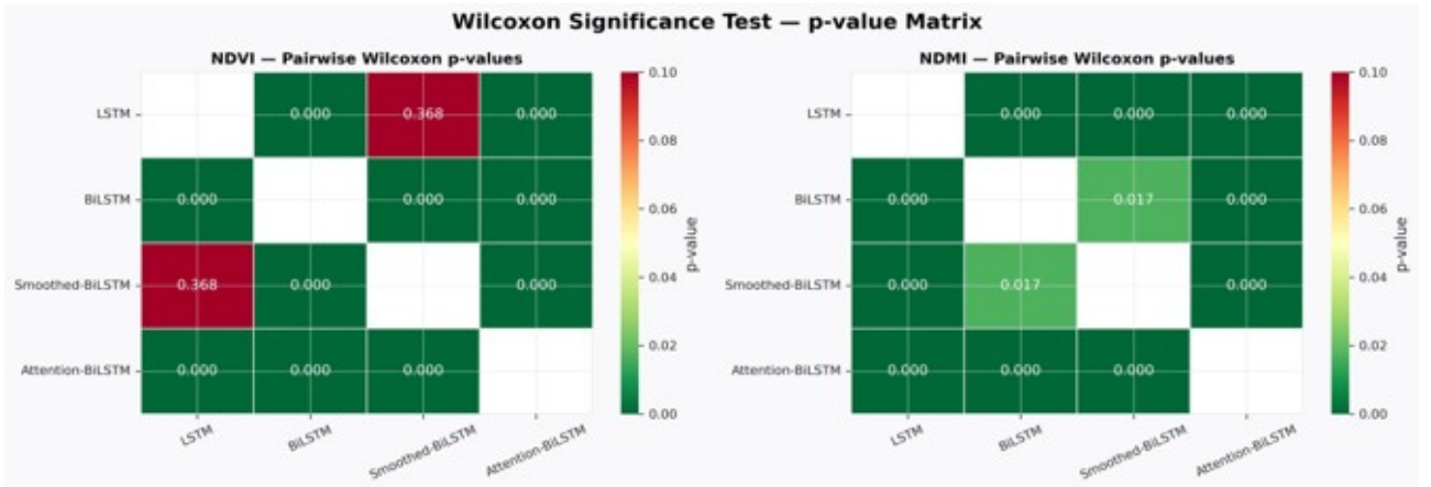
Figure 23: Pairwise Wilcoxon signed-rank test p-value matrices for NDVI (left) and NDMI (right). Green cells ( p < 0.05 ) indicate statistically significant performance differences; red cells indicate non-significant differences. All off-diagonal p-values of 0.000 represent p < 0.0001 .
