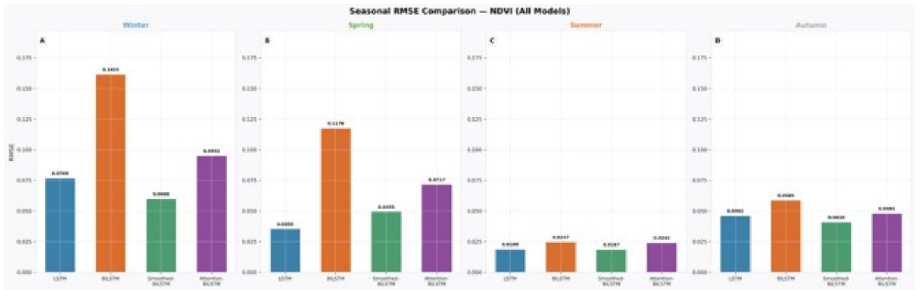
Figure 18: Seasonal RMSE comparison for NDVI across all four models. Panels show (A) winter, (B) spring, (C) summer, and (D) autumn seasonal performance.
