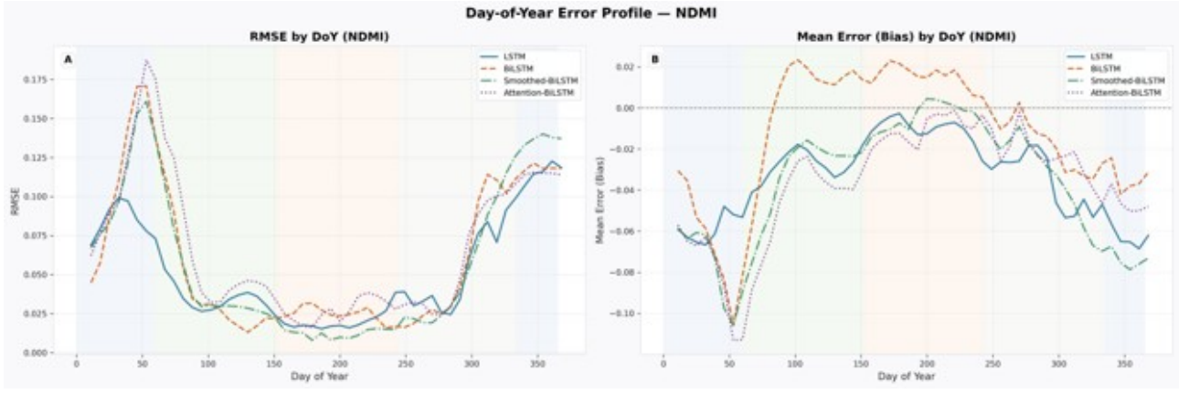
Figure 22: Day-of-Year error profiles for NDMI: (A) RMSE by DoY and (B) mean error (bias) by DoY. Note the rising RMSE trend from DoY 250 onward for Smoothed-BiLSTM and Attention-BiLSTM.
