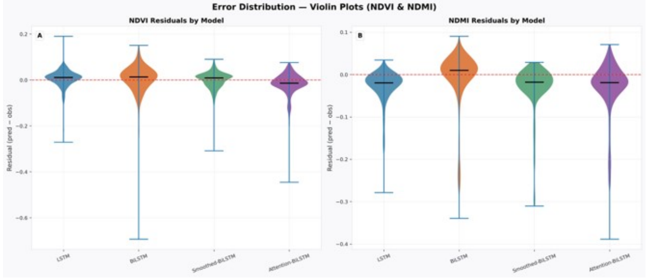
Figure 24: Violin plots of residual distributions (predicted – observed) for NDVI (A) and NDMI (B) across all four models.
