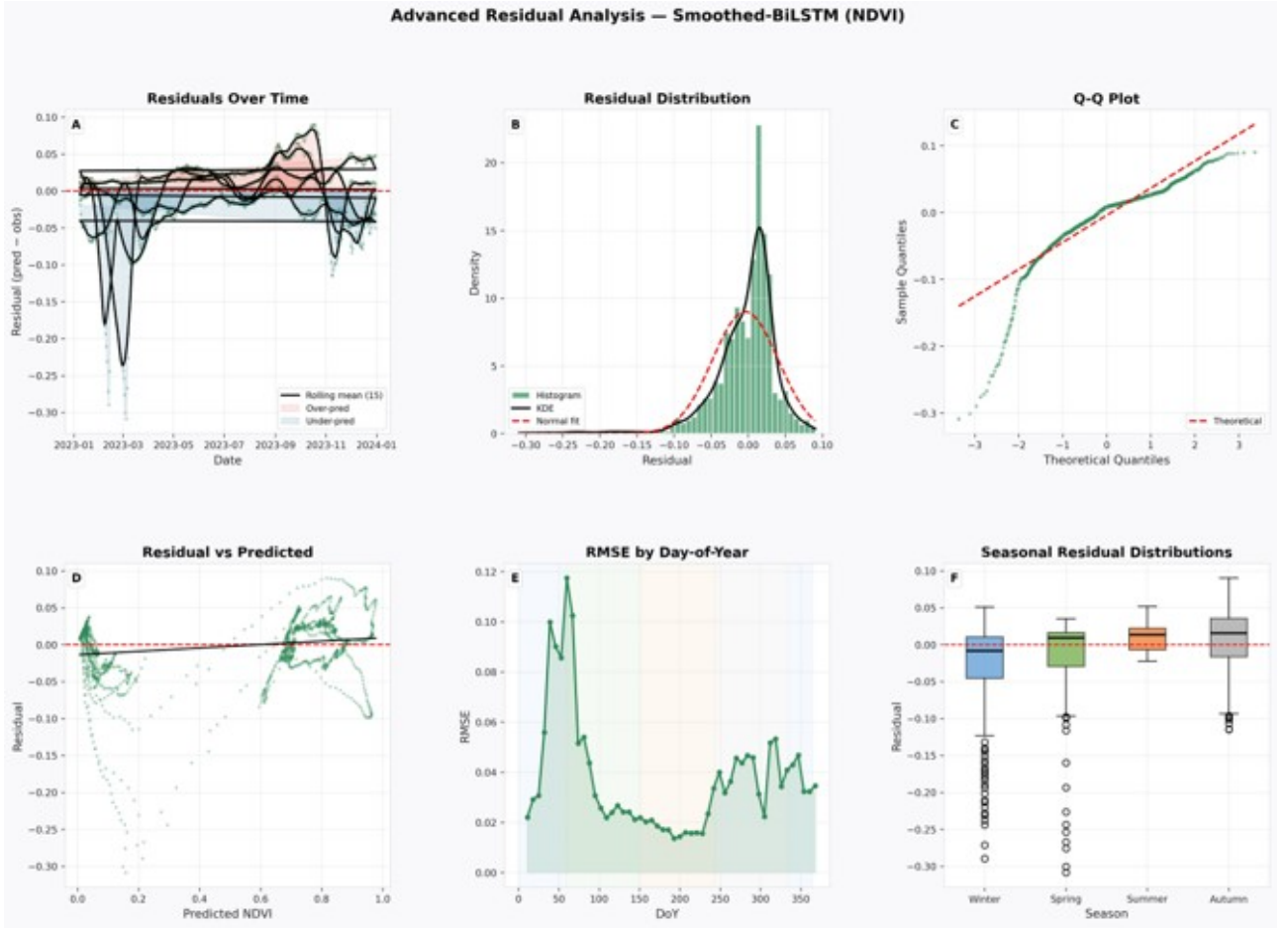
Figure 12: Advanced residual analysis for the Smoothed-BiLSTM (NDVI). Compared to the standard BiLSTM, residual spread is substantially reduced, with a near-symmetric distribution and improved seasonal error profile.
