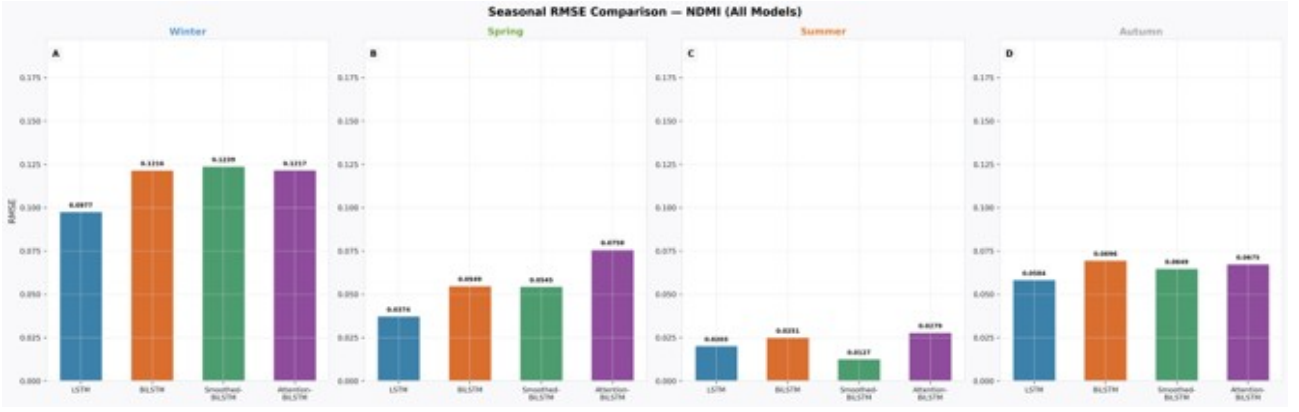
Figure 19: Seasonal RMSE comparison for NDMI across all four models. Winter RMSE values are uniformly high (0.098–0.124), whereas summer achieves minimum errors (0.013–0.028).
