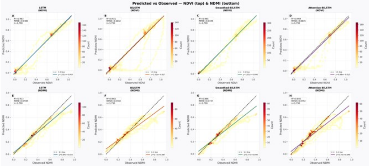
Figure 9: Density scatter plots of predicted versus observed values for NDVI (A–D) and NDMI (E–H) across all four architectures.
