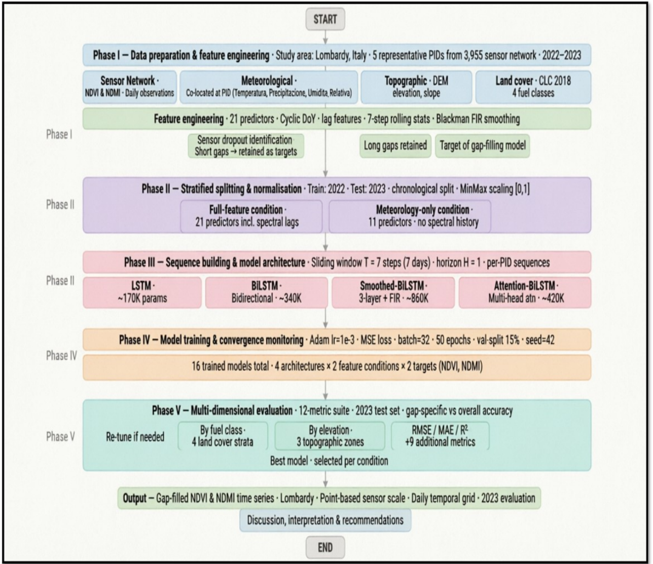
Figure 2: Full Methodological Flowchart
