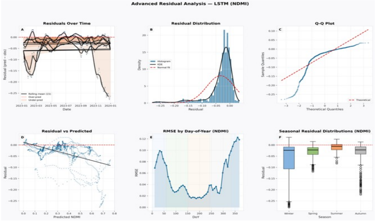
Figure 14: Advanced residual analysis for the LSTM (NDMI). Consistent under-prediction bias is apparent in panels A and F, with residuals concentrated in the range [-0.25, 0.05] .
