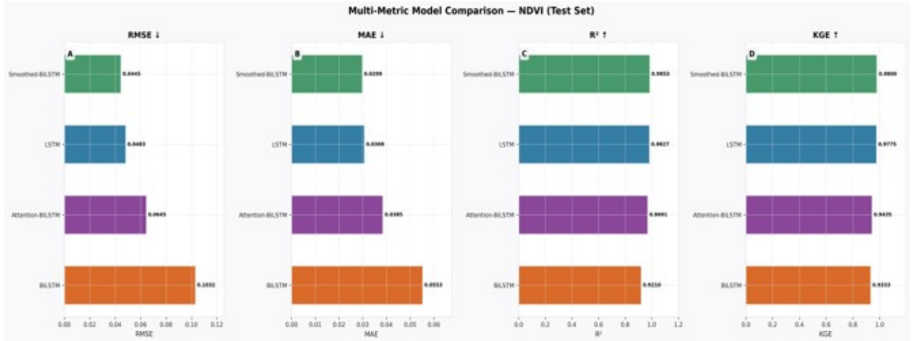
Figure 6: Multi-metric model comparison for NDVI prediction on the test set ( n = 1,790 ), showing RMSE (A), MAE (B), R^2 (C), and KGE (D).
