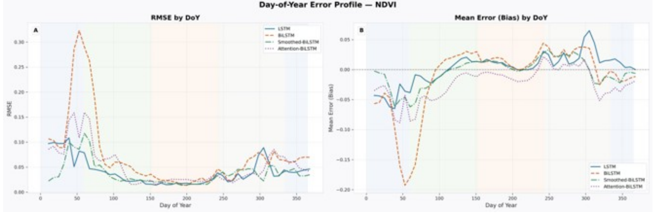
Figure 21: Day-of-Year (DoY) error profiles for NDVI: (A) RMSE by DoY and (B) mean error (bias) by DoY for all four models. Seasonal background colours indicate winter (blue), spring (green), summer (orange), and autumn (grey).
