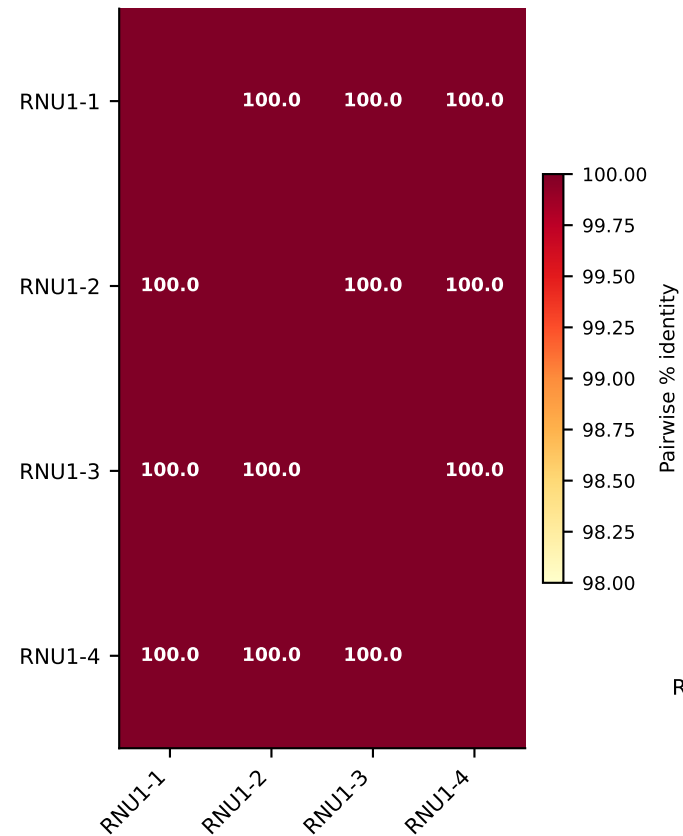
A RNU1 family (MANE Select, 4 loci)
