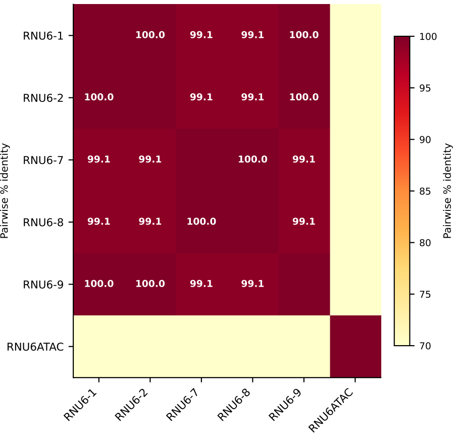
B RNU6 family (MANE Select, 6 loci)
