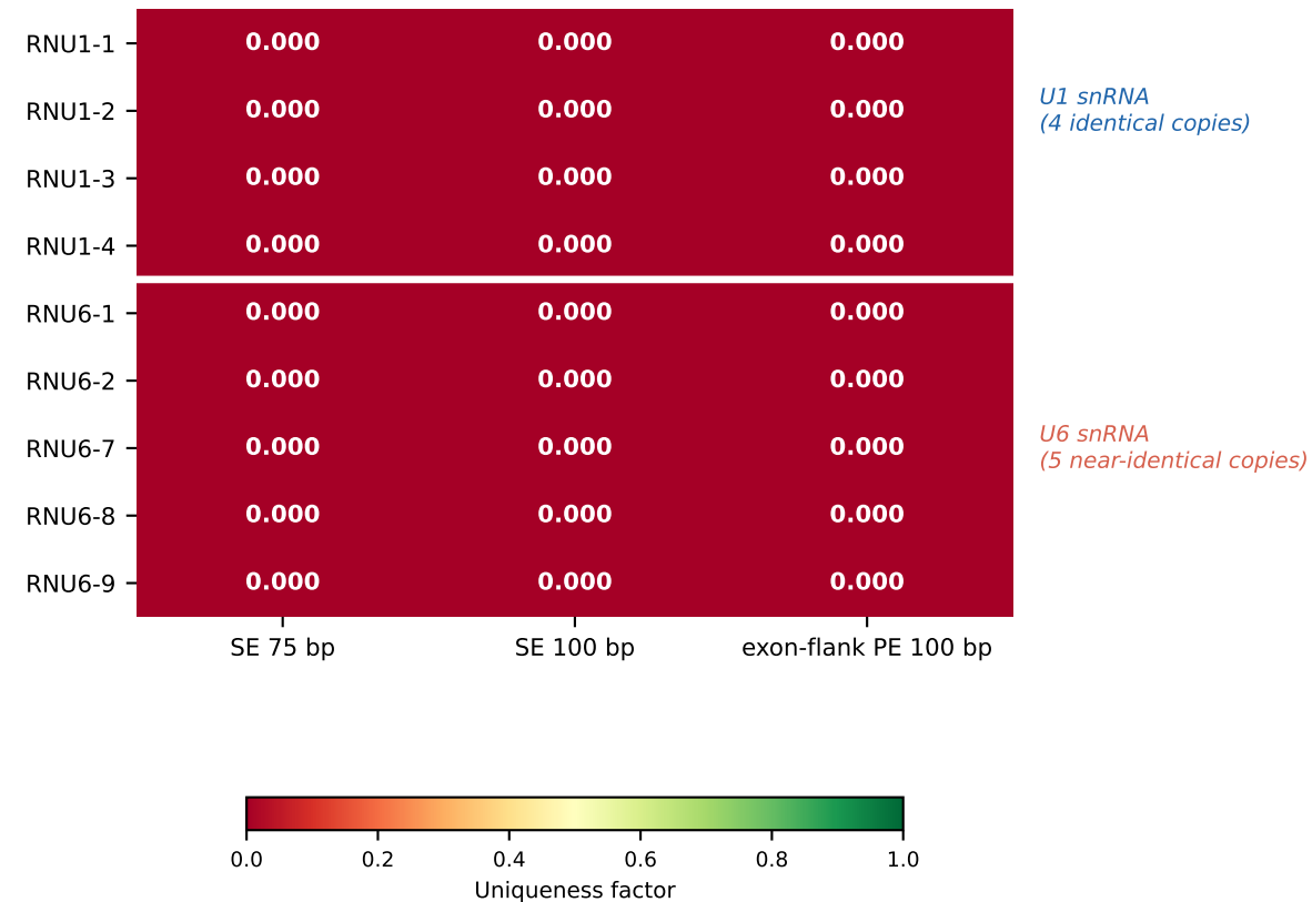
C Uniqueness factor — 3 simulation settings (MANE reference; reads from MANE RNA)
