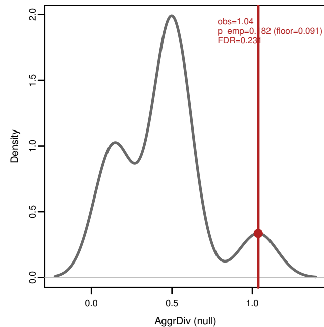
T0 (n=3 v 2, pool=5)
