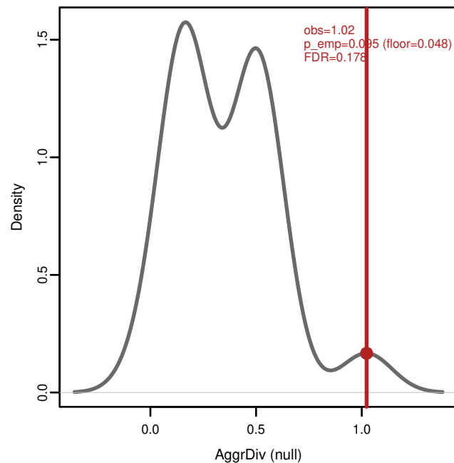
T1 (n=3 v 3, pool=6)
