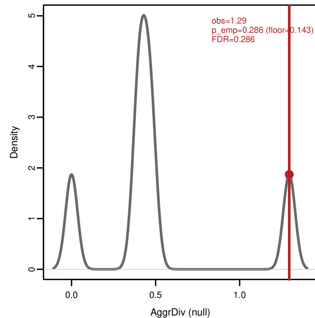
T6 (n=2 v 2, pool=4)
