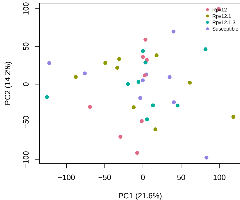
DESeq2 NB Pearson residuals – condition
