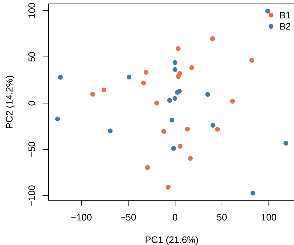
DESeq2 NB Pearson residuals – batch
