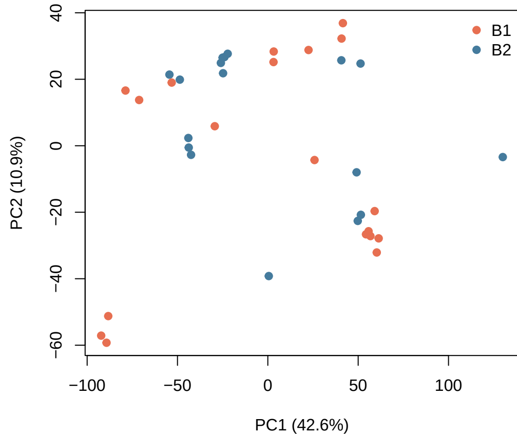
VST batch-adjusted visualization – batch
