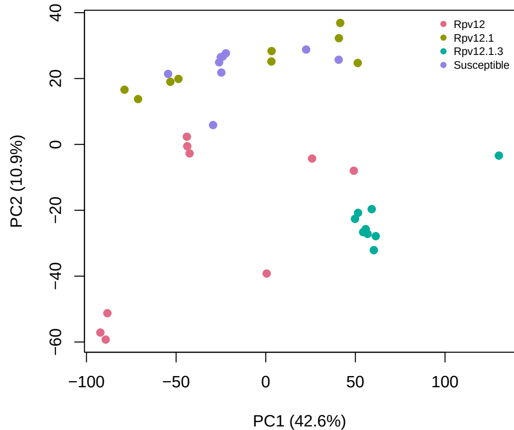
VST batch-adjusted visualization – condition
