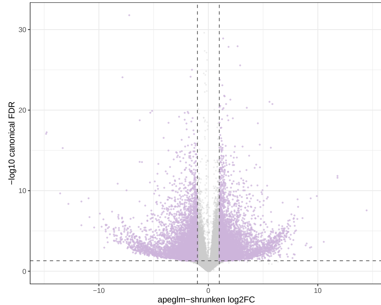
Volcano: newly called DE genes
