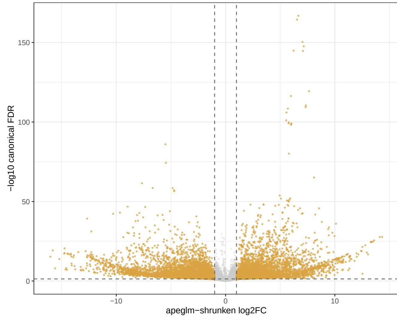
Volcano: shared DE genes
