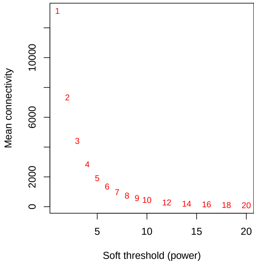
Mean connectivity
