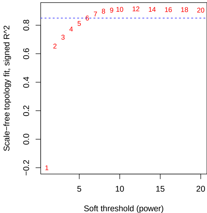
Scale independence
