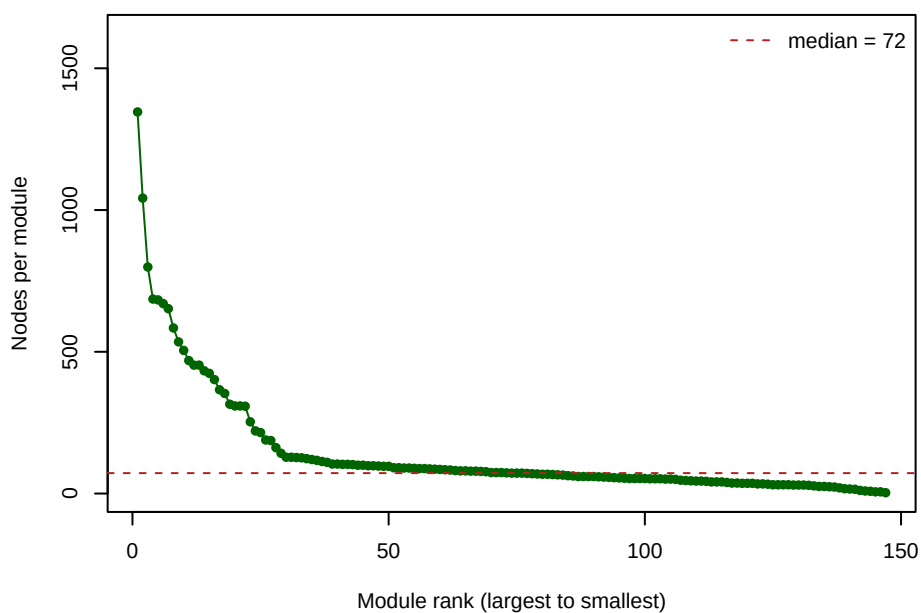
Original method – protected ComBat (147 modules)
