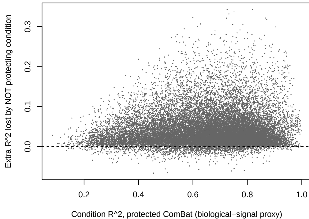
Leading-signal test: \rho=0.024 , p=7.66e-05
