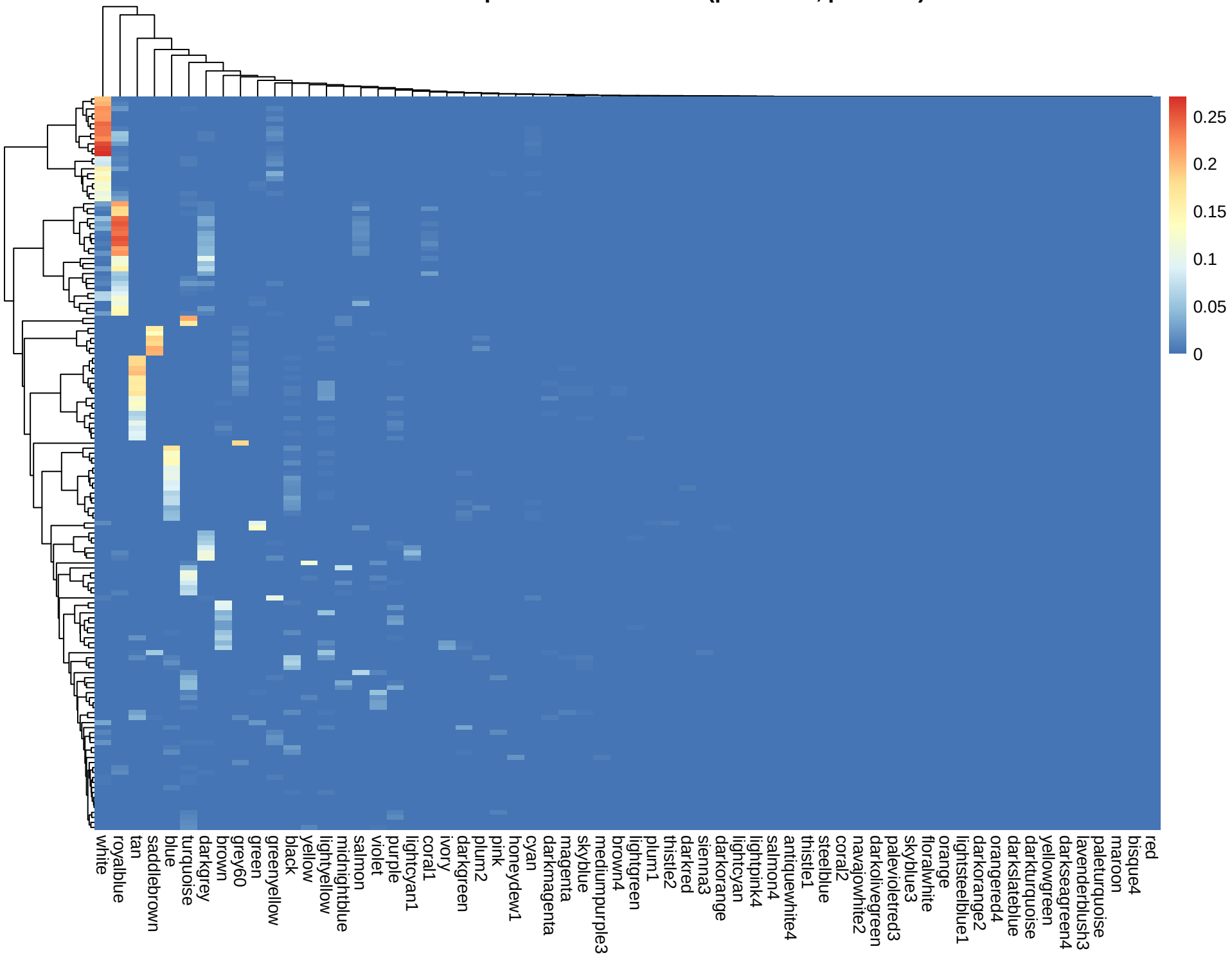
Jaccard overlap: GCNA vs WGCNA (protected, power12)
