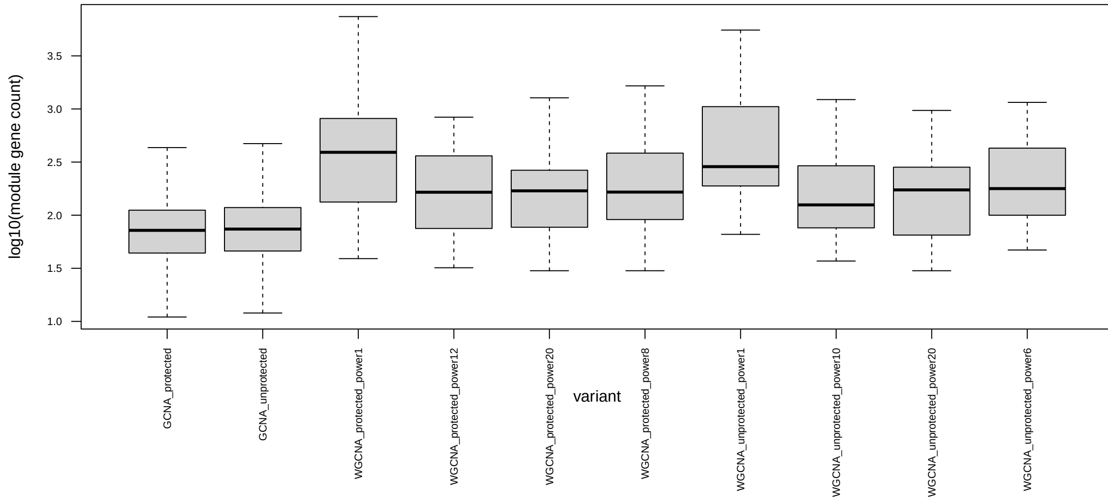
Module size distribution by method/ComBat setting
