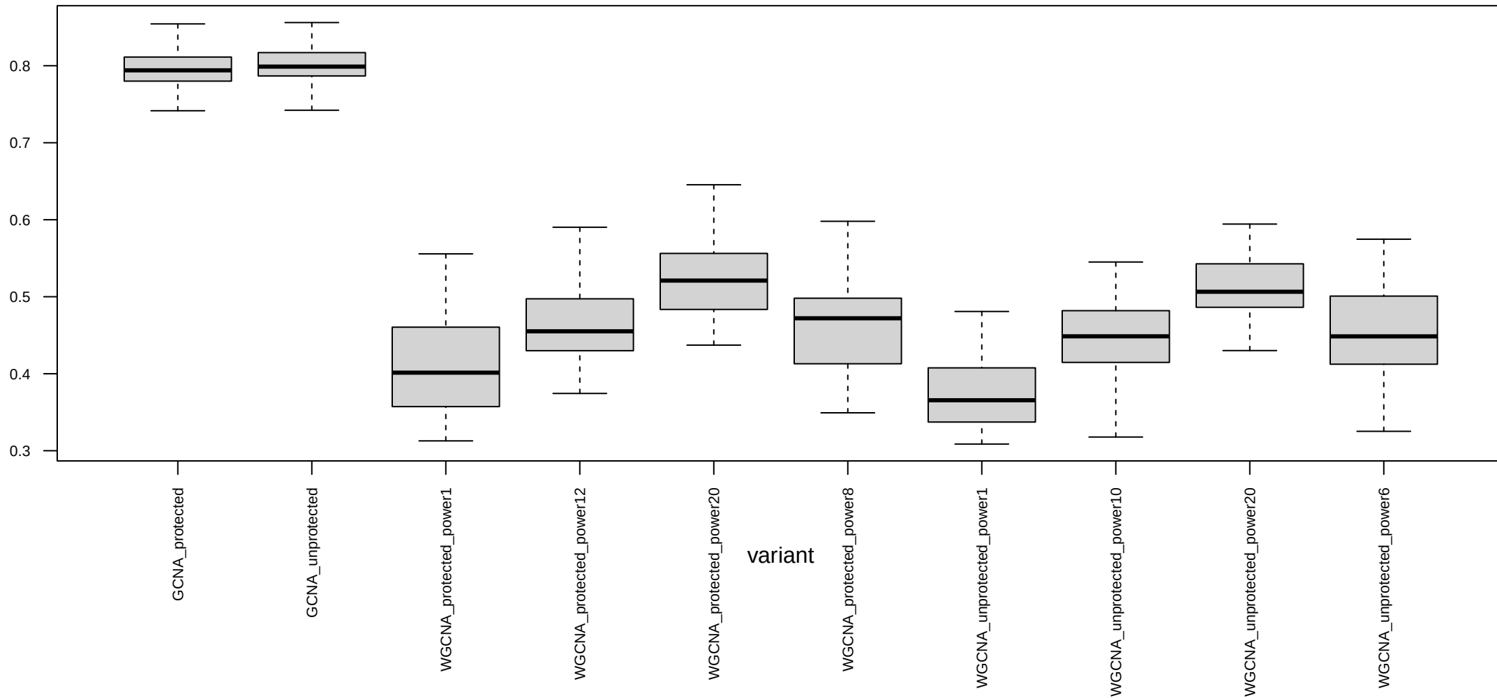
Within-module node correlation by method/ComBat setting
