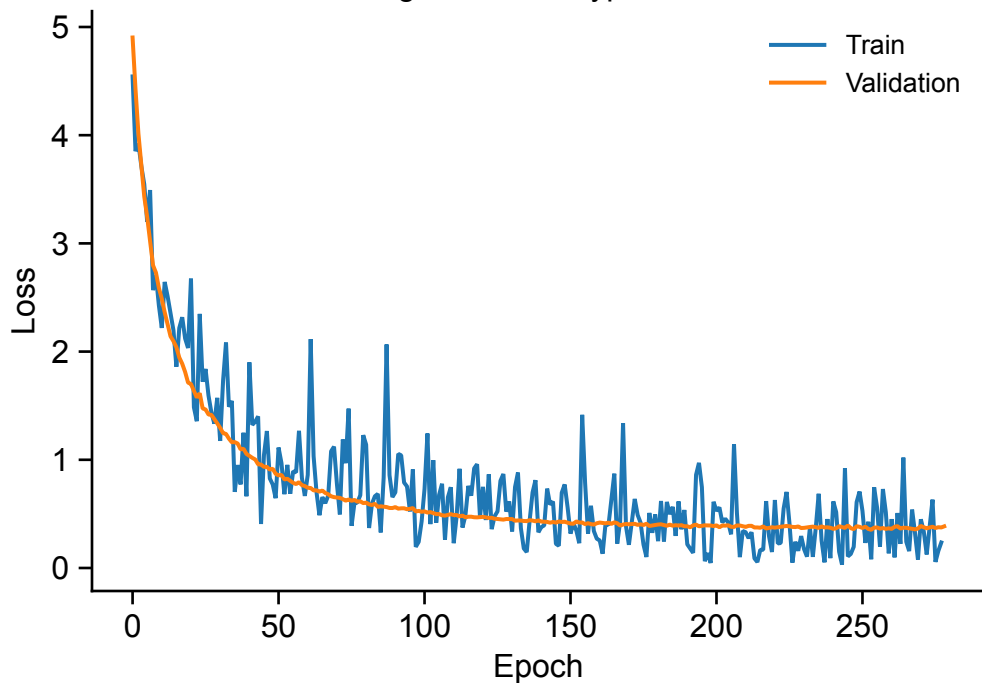
Training loss – Cell type classifier
