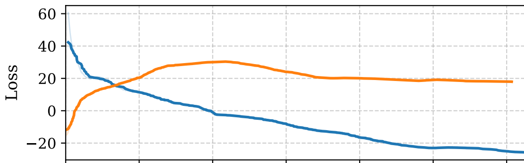
Critic Loss
