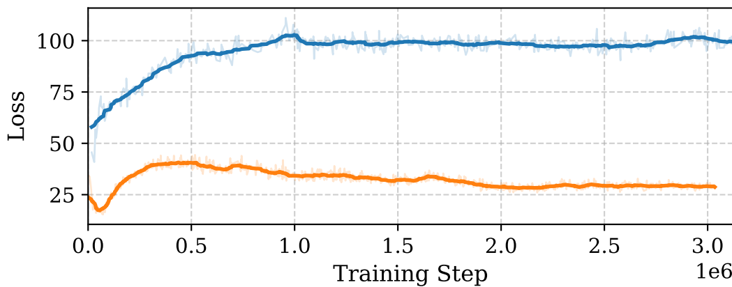
Critic Loss
