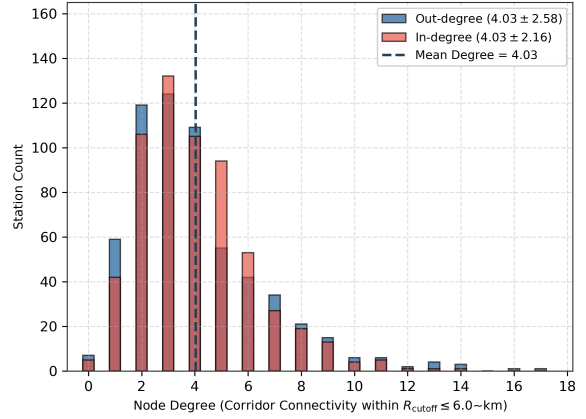
(b) Node Degree Distribution ( N = 608 Stations, |E| = 2,450 )
