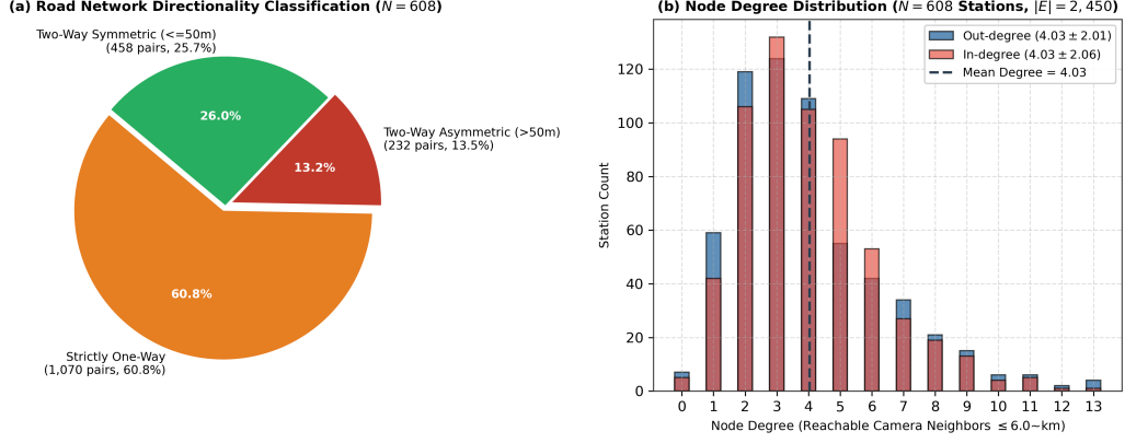
Figure 4: Topological characteristics of the empirical directed road graph: (a) Road network directionality classification into unidirectional links without reverse edges (60.8%), two-way asymmetric ( > 50 m, 13.5%), and two-way symmetric ( \leq 50 m, 25.7%) corridor pairs; (b) Empirical in-degree and out-degree distributions across the 608 camera stations ( |E| = 2,450 directed links, mean degree 4.03 \pm 2.16 in-degree and 4.03 \pm 2.58 out-degree).
