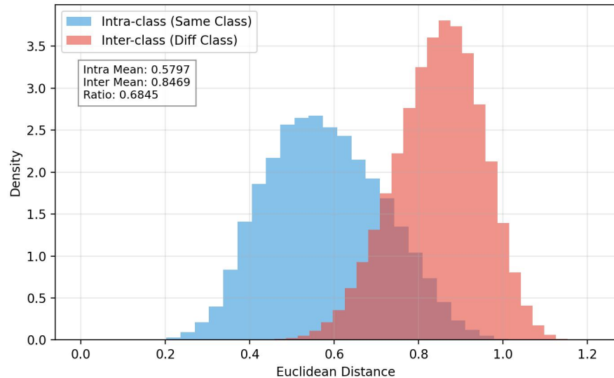
Distance Distribution Before Training
