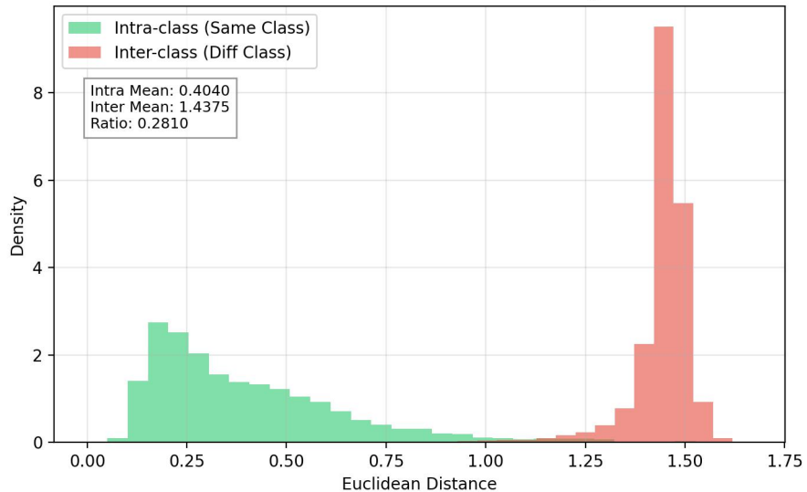
Distance Distribution After Training
