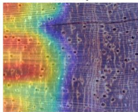
Before Training
