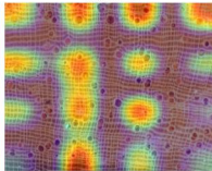
Before Training
