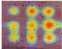
After Training
