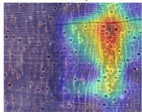
After Training
