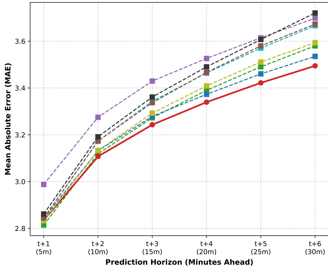
MAE Growth across Prediction Horizons
