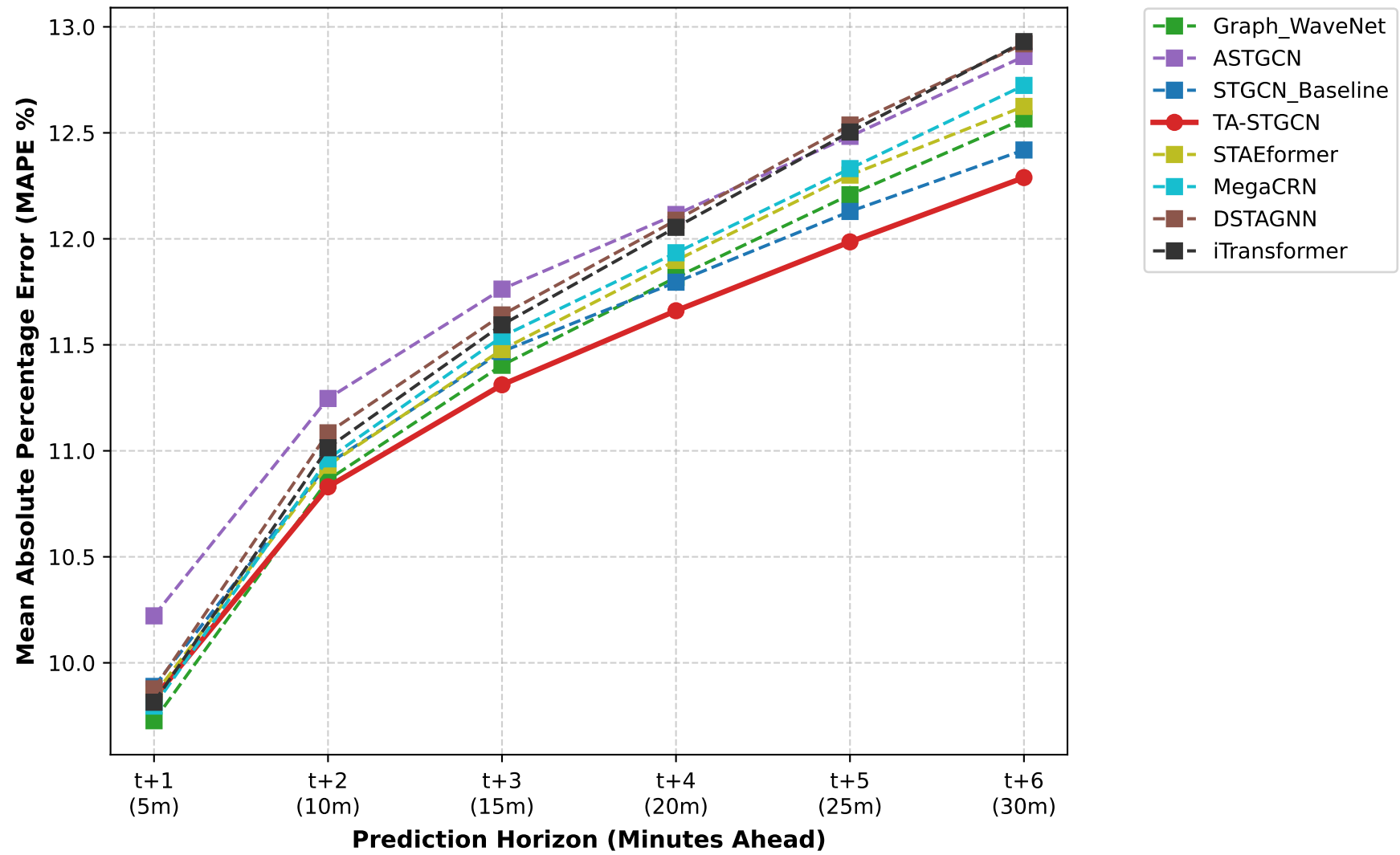
MAPE Growth across Prediction Horizons
