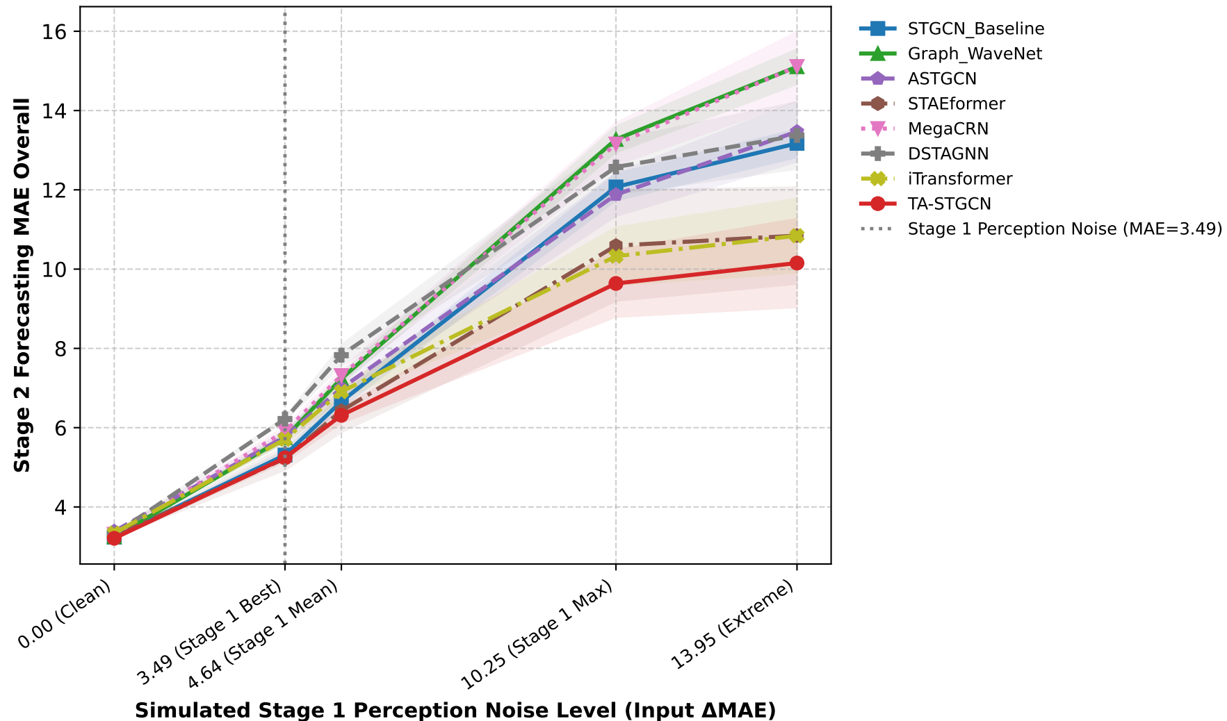
Robustness to Stage 1 Perception Noise Across All Models
