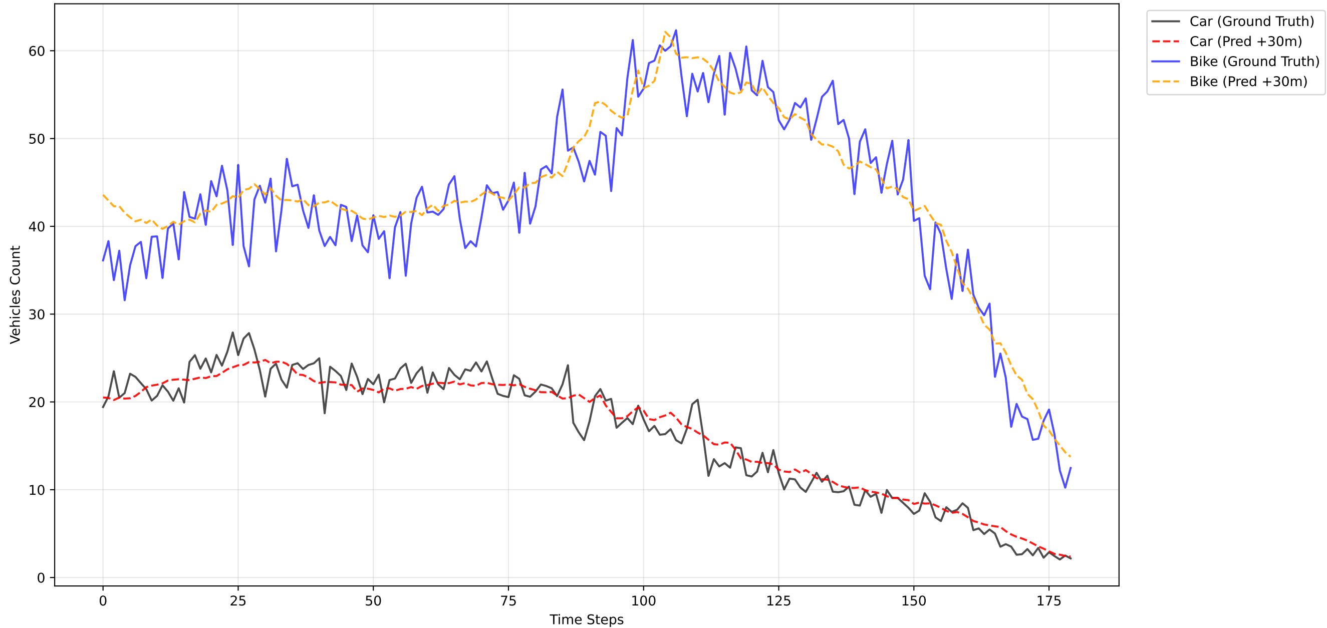
Node 26 - MAE Car: 1.35, MAE Bike: 2.88 (Prediction 30 mins ahead)
