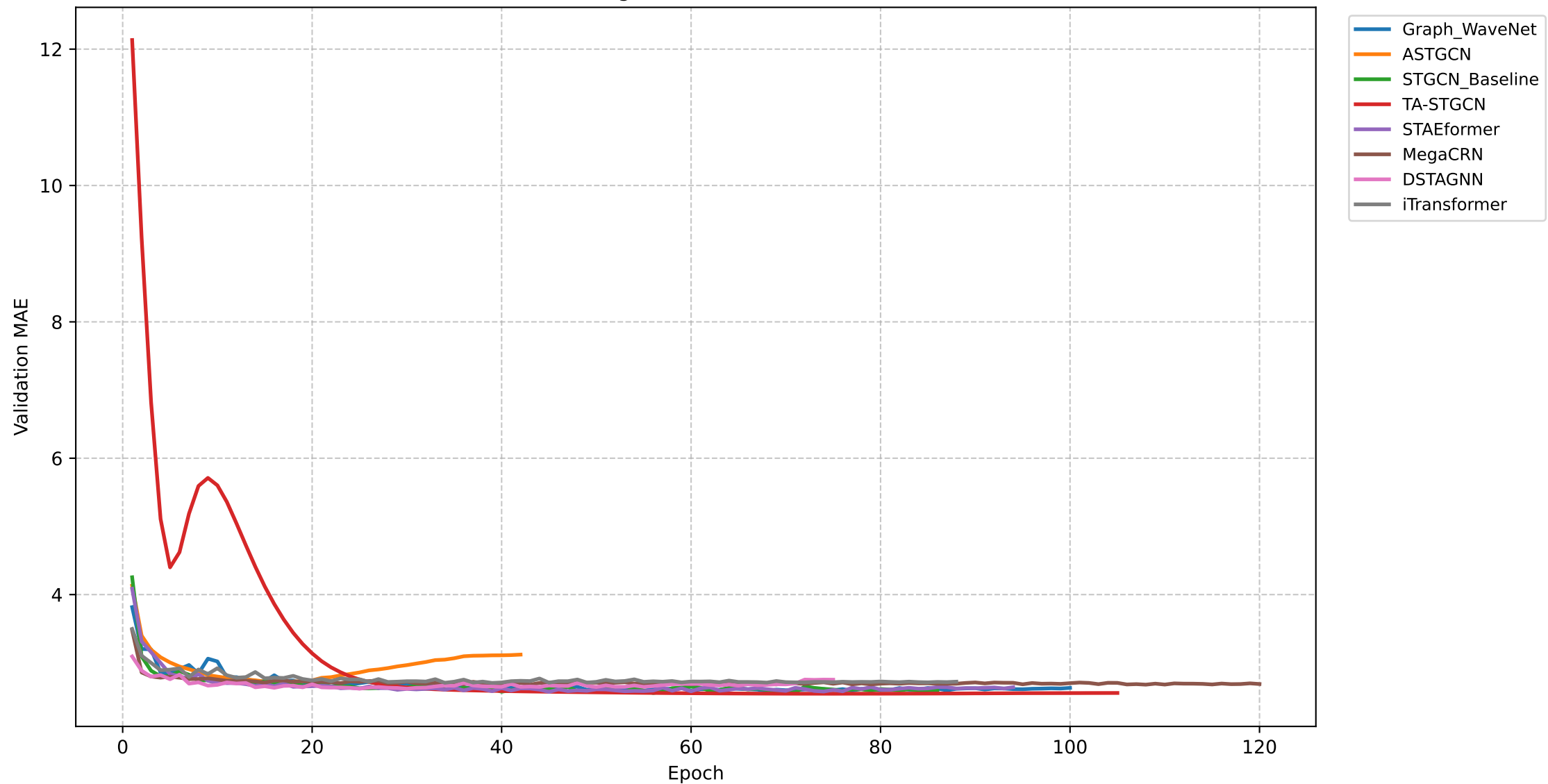
Validation MAE Convergence Curves (Main SOTA Baselines)
