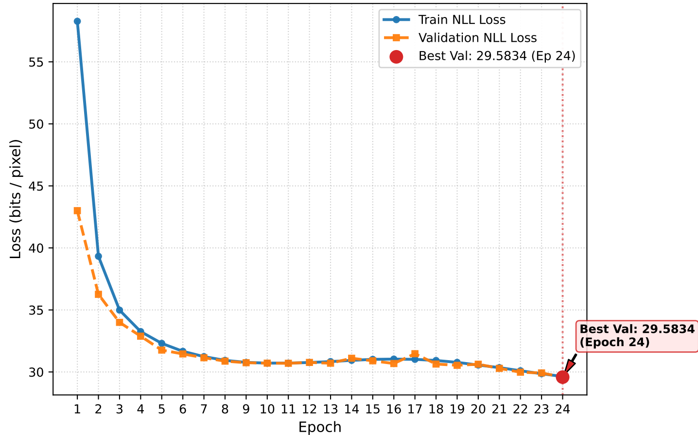
Total Negative Log-Likelihood (NLL) Loss
