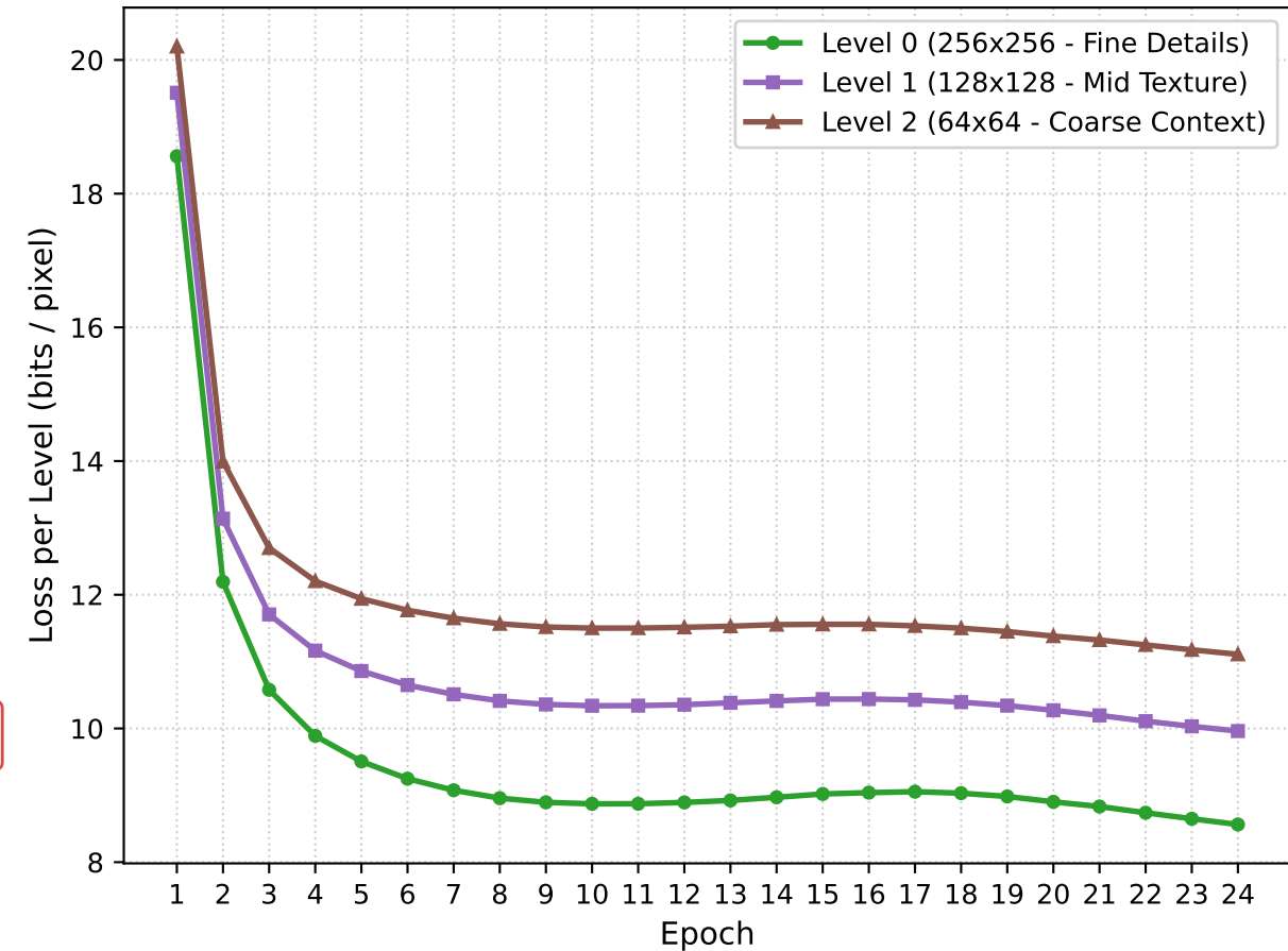
Multi-Scale Pyramid NLL Loss Breakdown
