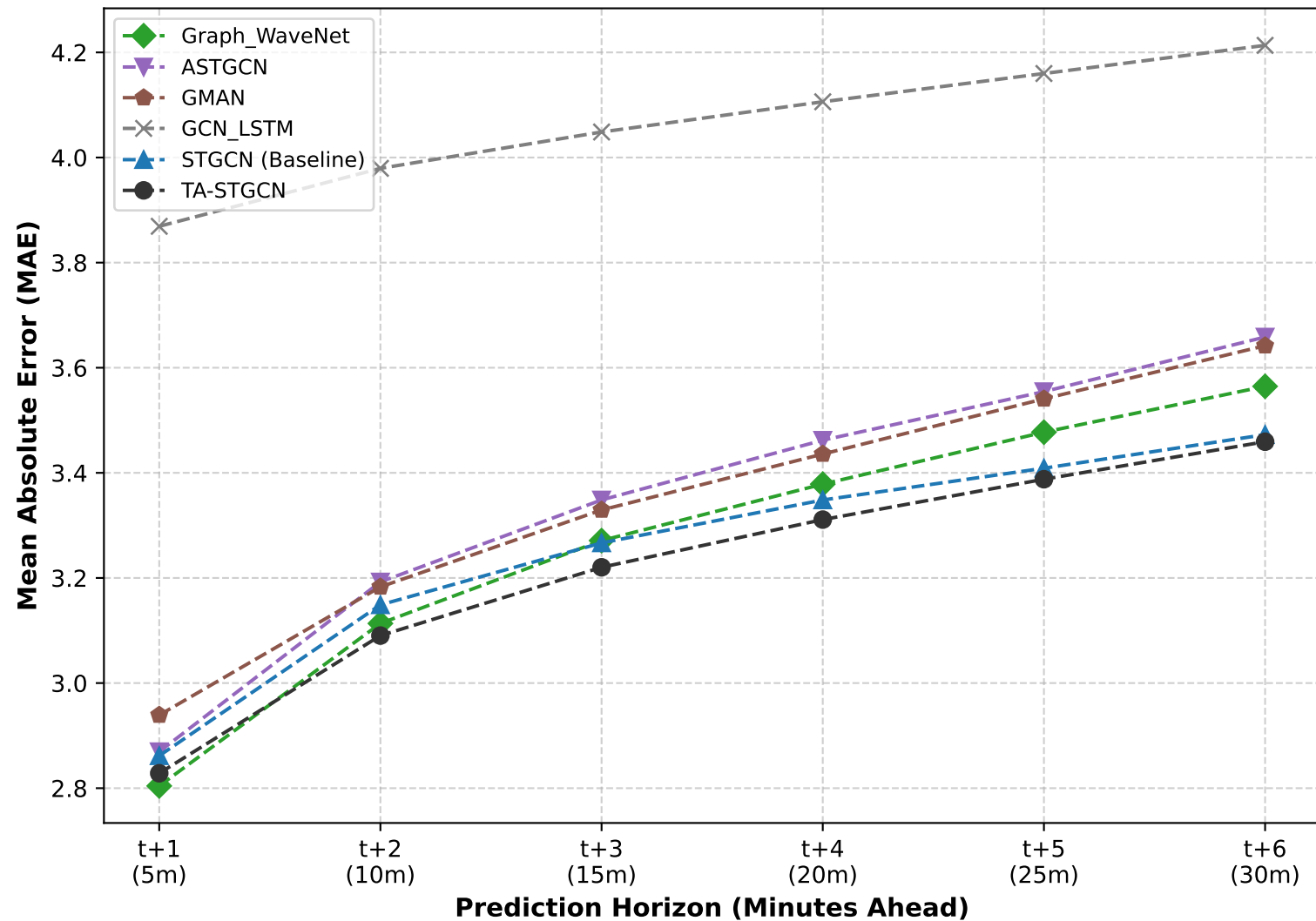
(a) MAE Growth across Prediction Horizons
