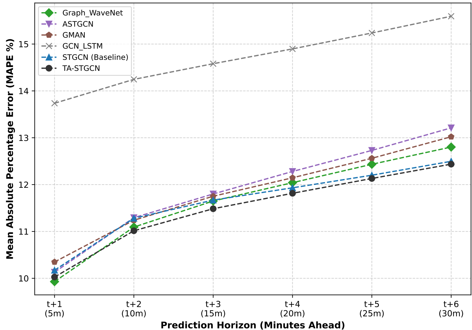
(b) MAPE Growth across Prediction Horizons
