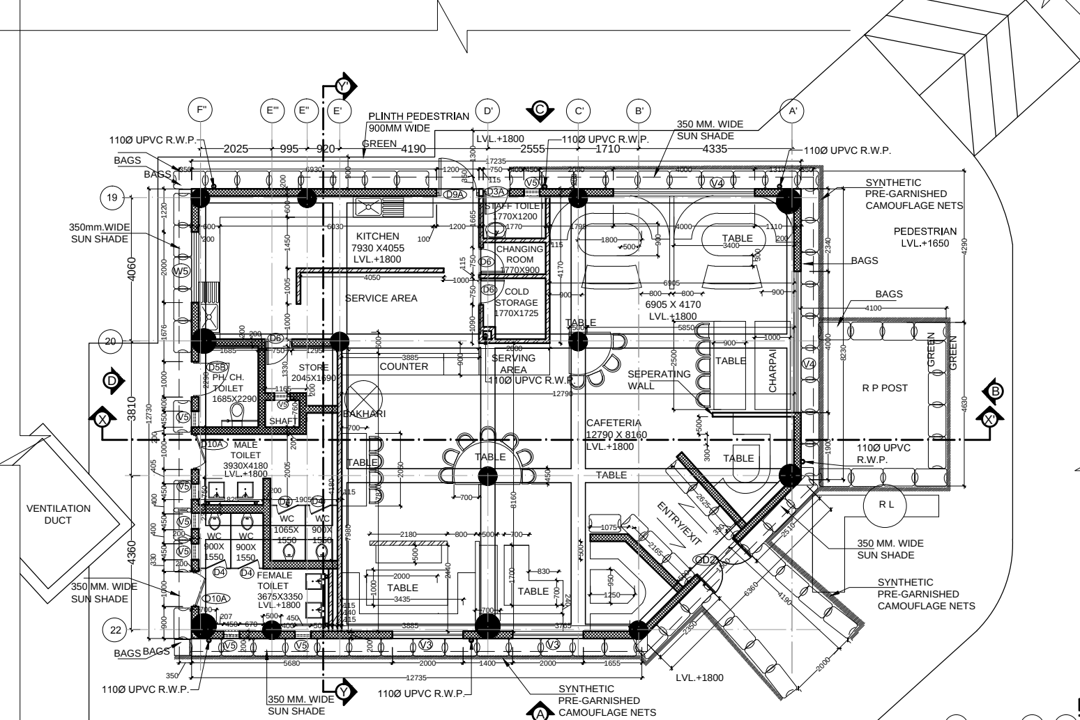
CAFETERIA (GROUND FLOOR PLAN)
