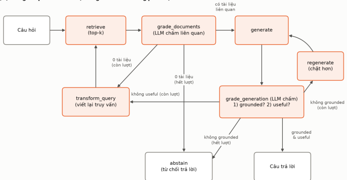
(b) LangGraph Self-RAG (trung bình 7.6 lần gọi LLM)
