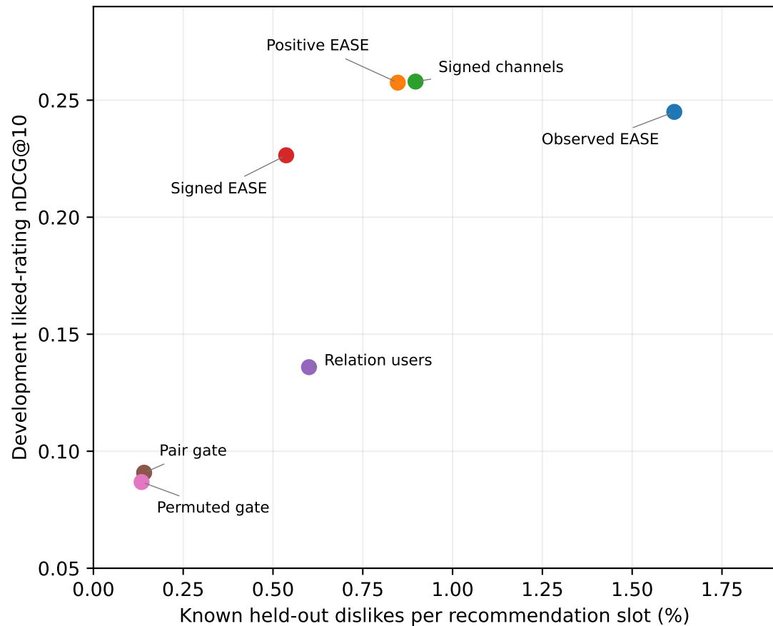
Avoiding observed dislikes does not guarantee relevance
