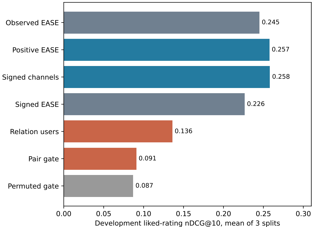
Contrast models underperform the linear controls
