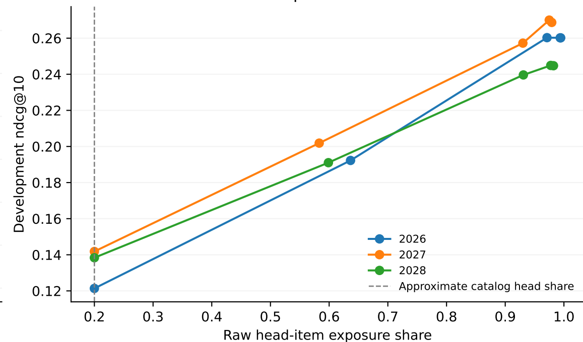
Item-exposure trade-off
