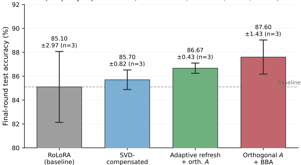
QNLI proxy improvements (RoBERTa-base, 50 clients, rank 4, \text{lr } 10^{-2} )
