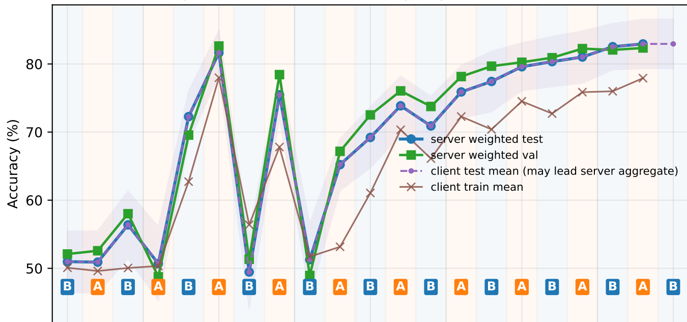
Orthogonal-A default alternation proxy QNLI C50 r4 seed0
