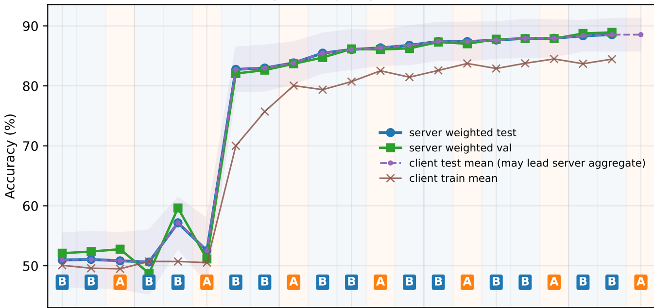
BBA + orthogonal-A proxy QNLI C50 r4 seed0
