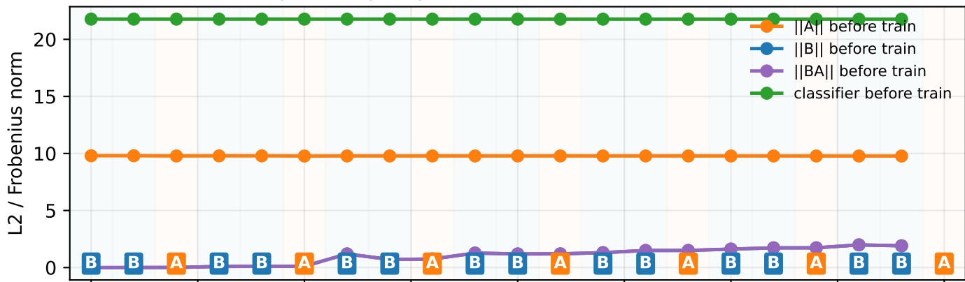
BBA + orthogonal-A proxy QNLI C50 r4 seed0: internal factor norms
