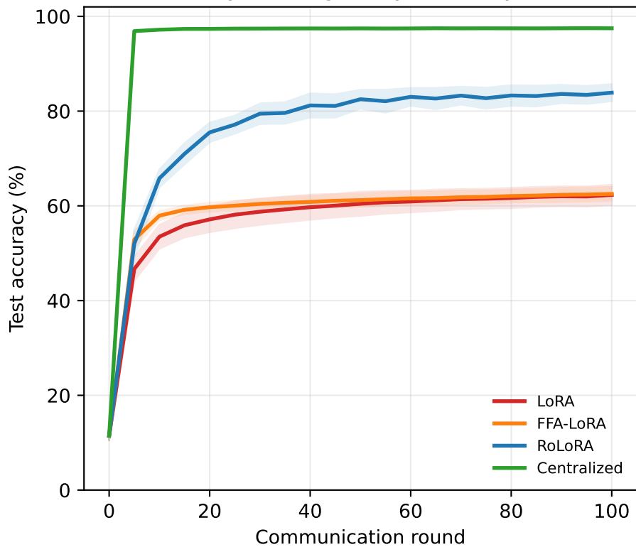
Toy heterogeneity accuracy
