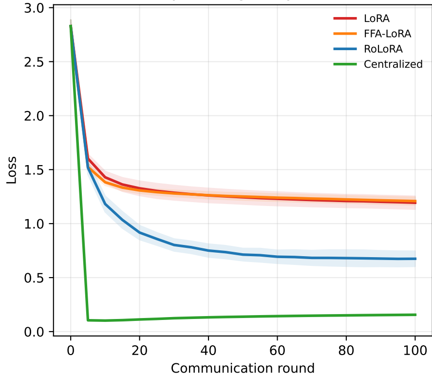
Toy heterogeneity loss
