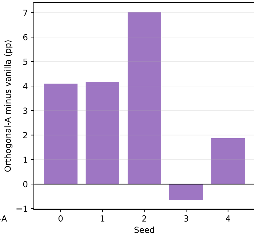
Per-seed delta
